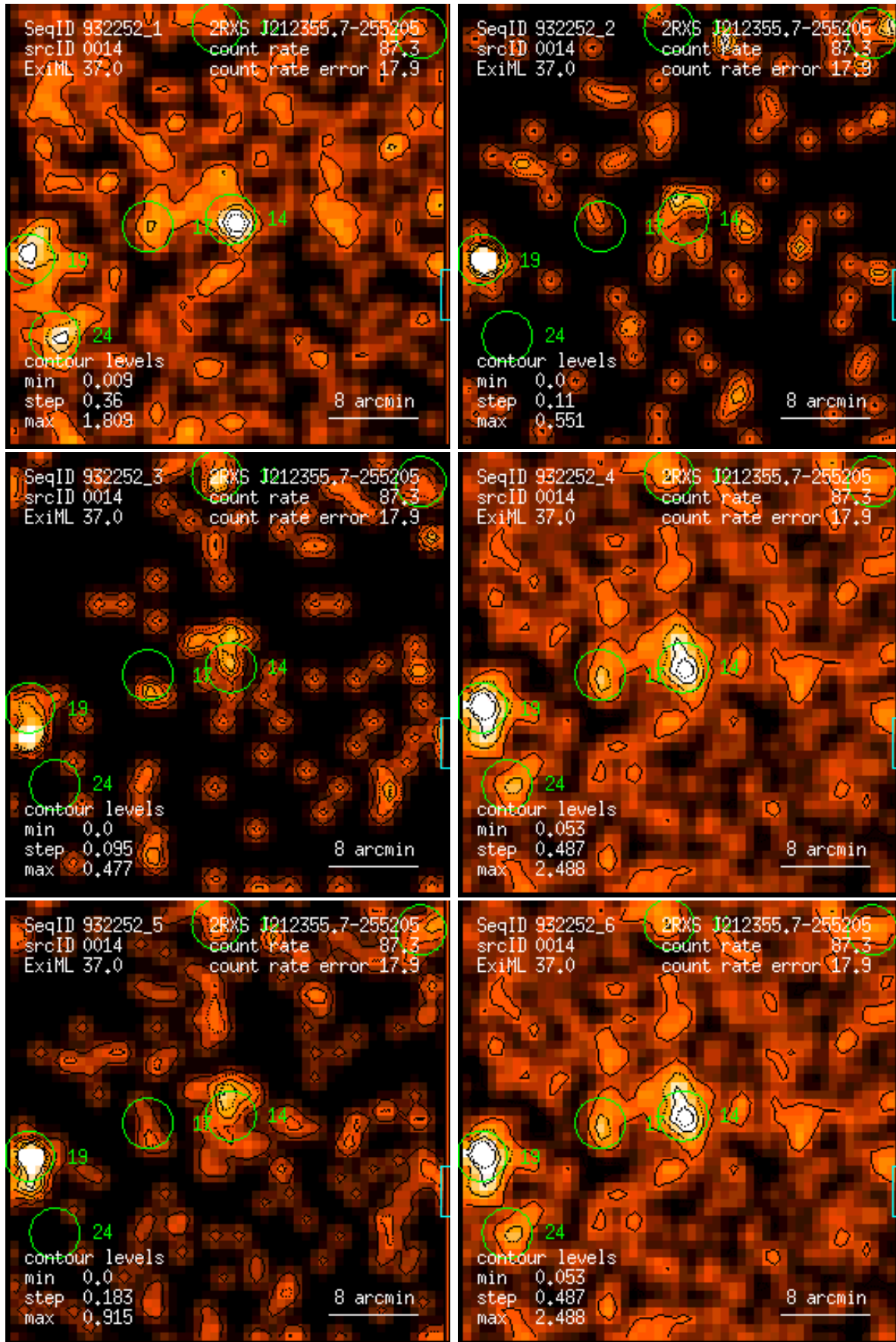
Figure 14: RASS 932252: detection 0014: band rate images, Gaussian filter: (1) PSPC channels 11 – 41, (2) 52 – 90, (3) 91 – 201, (4) 11 – 235, (5) 52 – 201, (6) 11 – 201. Broad band rates in counts/ks. Band rate contour levels in counts/ks/arcmin 2 .
