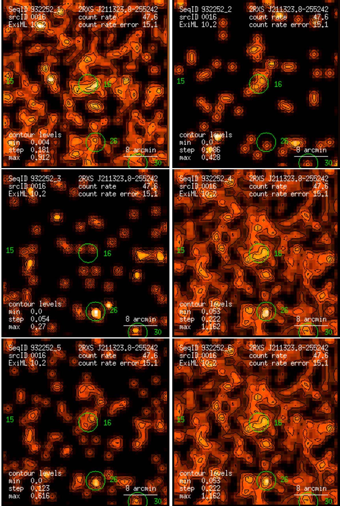
Figure 16: RASS 932252: detection 0016: band rate images, Gaussian filter: (1) PSPC channels 11 – 41, (2) 52 – 90, (3) 91 – 201, (4) 11 – 235, (5) 52 – 201, (6) 11 – 201. Broad band rates in counts/ks. Band rate contour levels in counts/ks/arcmin 2 .
