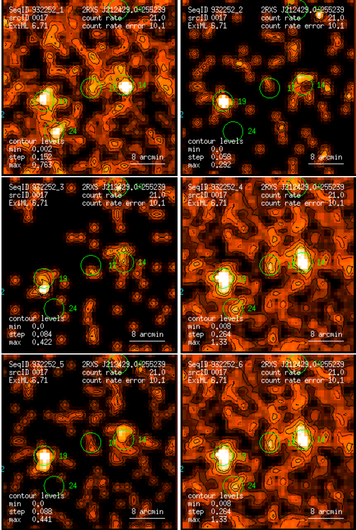
Figure 17: RASS 932252: detection 0017: band rate images, Gaussian filter: (1) PSPC channels 11 – 41, (2) 52 – 90, (3) 91 – 201, (4) 11 – 235, (5) 52 – 201, (6) 11 – 201. Broad band rates in counts/ks. Band rate contour levels in counts/ks/arcmin 2 .
