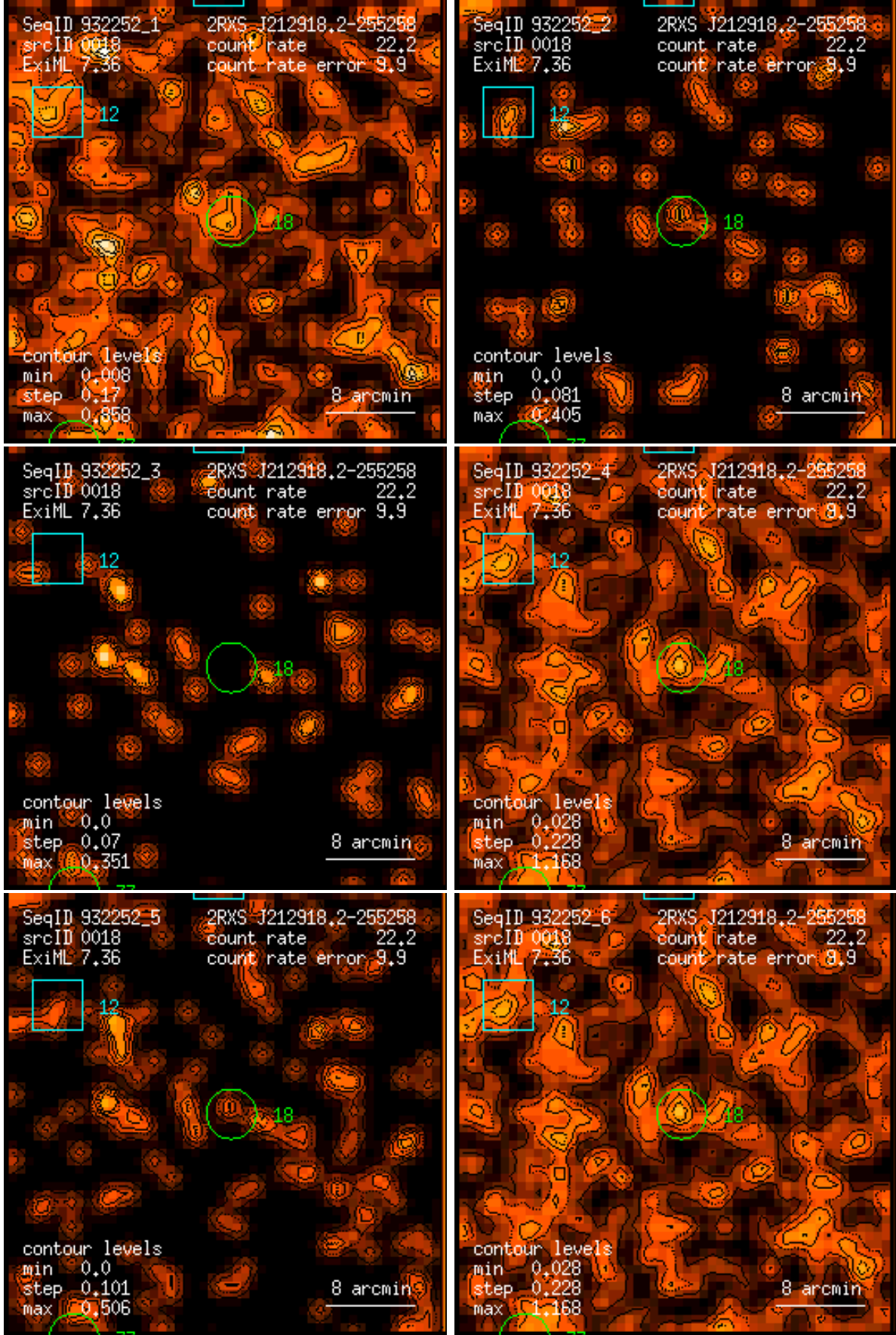
Figure 18: RASS 932252: detection 0018: band rate images, Gaussian filter: (1) PSPC channels 11 – 41, (2) 52 – 90, (3) 91 – 201, (4) 11 – 235, (5) 52 – 201, (6) 11 – 201. Broad band rates in counts/ks. Band rate contour levels in counts/ks/arcmin 2 .
