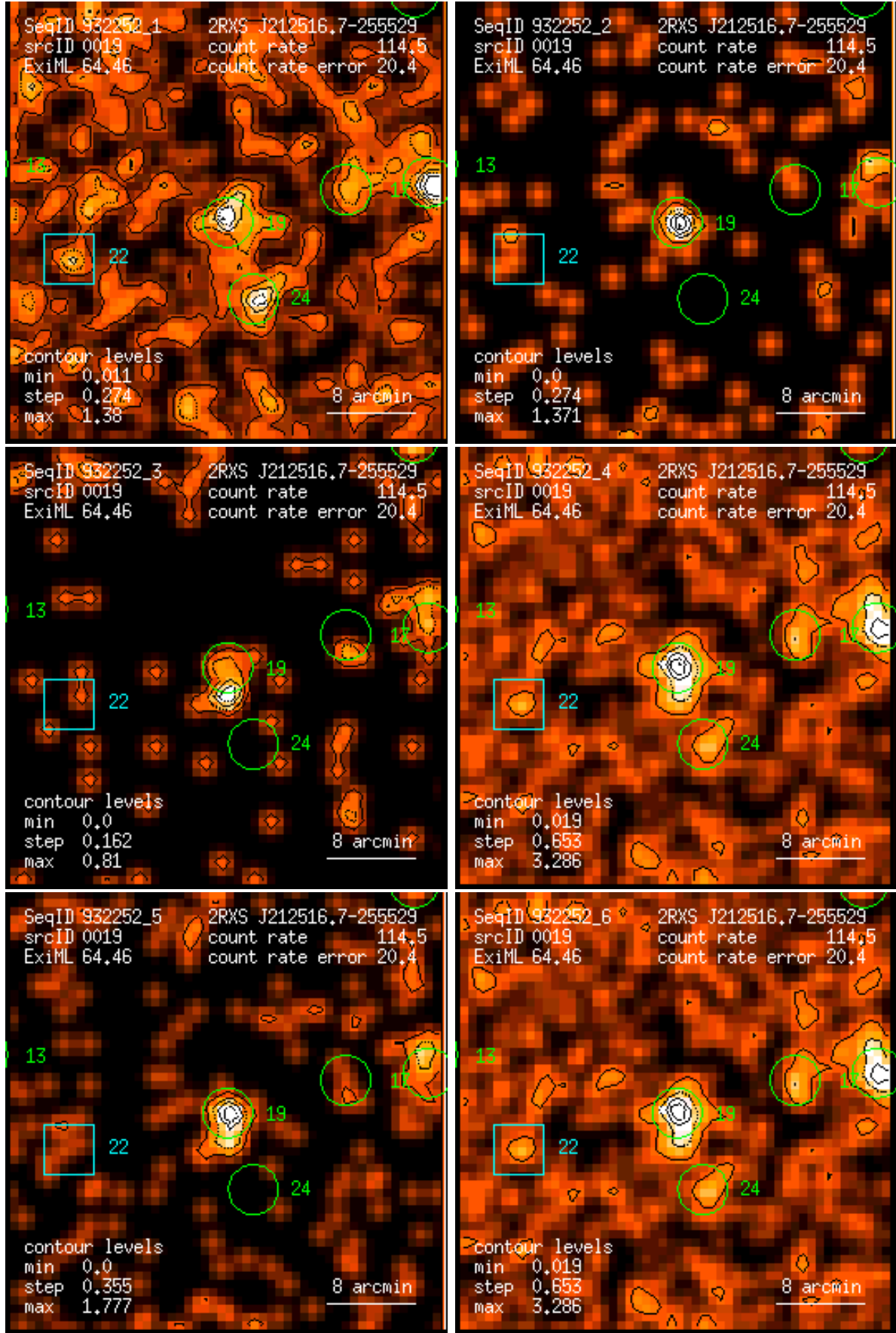
Figure 19: RASS 932252: detection 0019: band rate images, Gaussian filter: (1) PSPC channels 11 – 41, (2) 52 – 90, (3) 91 – 201, (4) 11 – 235, (5) 52 – 201, (6) 11 – 201. Broad band rates in counts/ks. Band rate contour levels in counts/ks/arcmin 2 .
