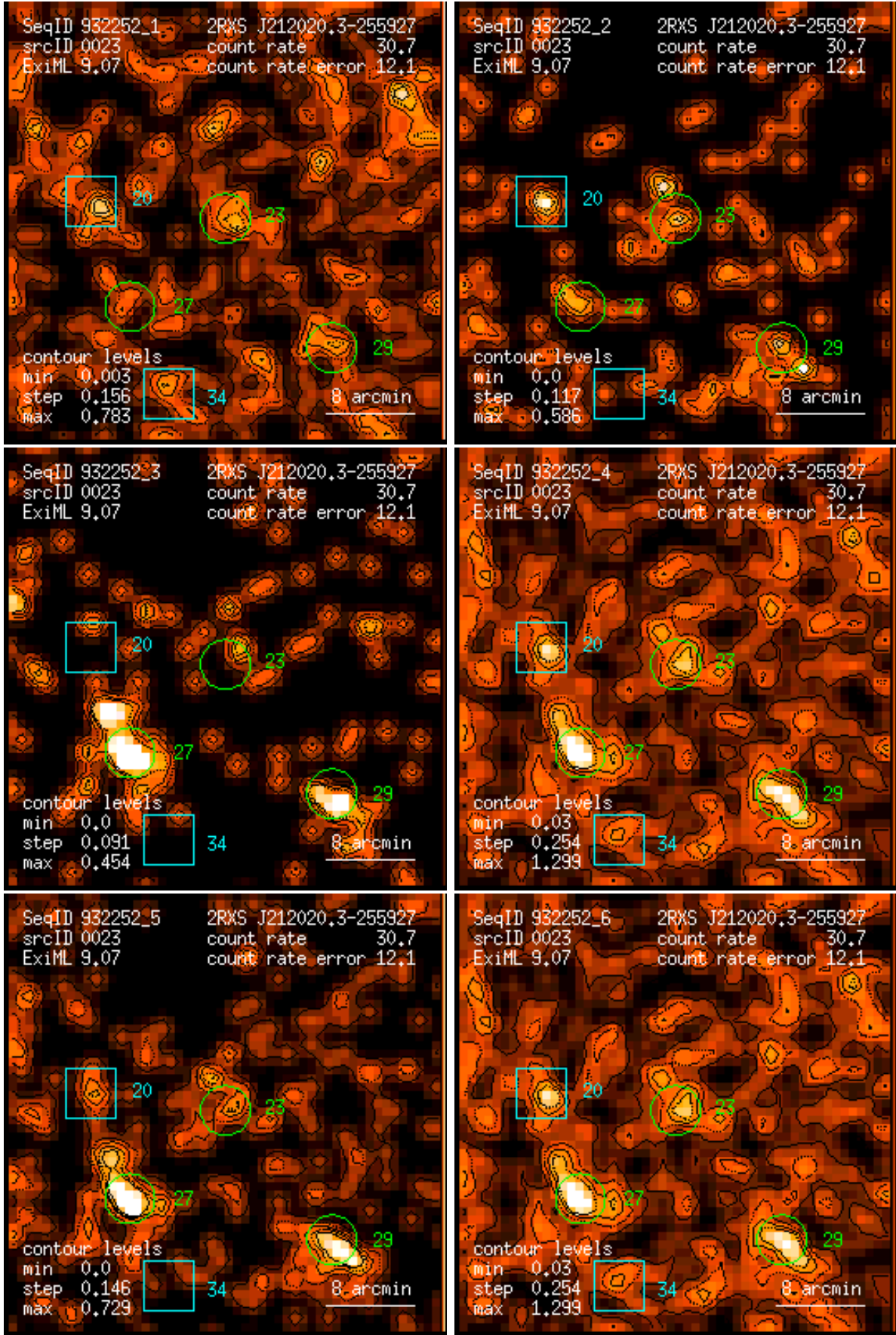
Figure 23: RASS 932252: detection 0023: band rate images, Gaussian filter: (1) PSPC channels 11 – 41, (2) 52 – 90, (3) 91 – 201, (4) 11 – 235, (5) 52 – 201, (6) 11 – 201. Broad band rates in counts/ks. Band rate contour levels in counts/ks/arcmin 2 .
