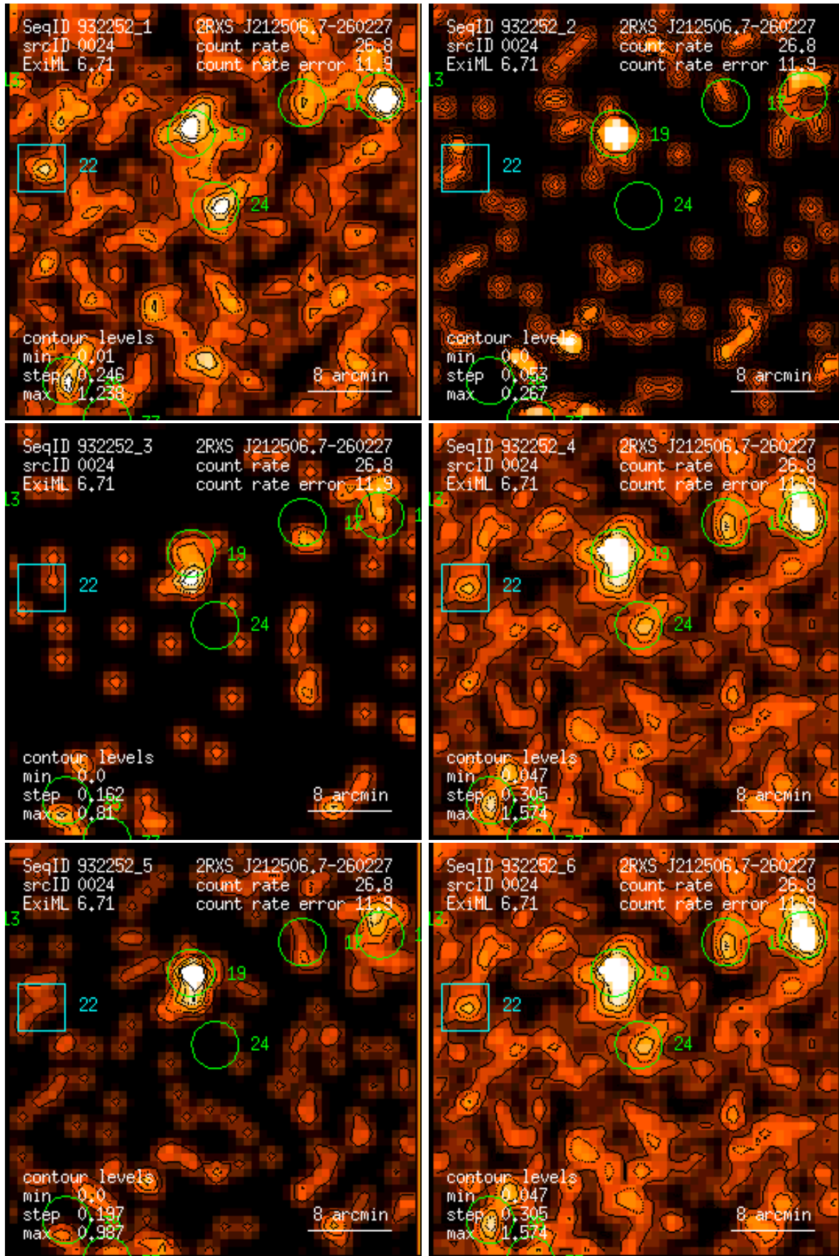
Figure 24: RASS 932252: detection 0024: band rate images, Gaussian filter: (1) PSPC channels 11 – 41, (2) 52 – 90, (3) 91 – 201, (4) 11 – 235, (5) 52 – 201, (6) 11 – 201. Broad band rates in counts/ks. Band rate contour levels in counts/ks/arcmin 2 .
