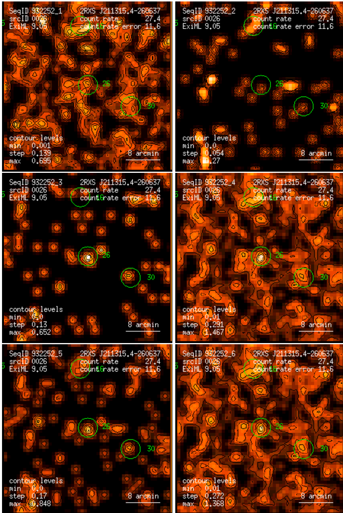
Figure 26: RASS 932252: detection 0026: band rate images, Gaussian filter: (1) PSPC channels 11 – 41, (2) 52 – 90, (3) 91 – 201, (4) 11 – 235, (5) 52 – 201, (6) 11 – 201. Broad band rates in counts/ks. Band rate contour levels in counts/ks/arcmin 2 .
