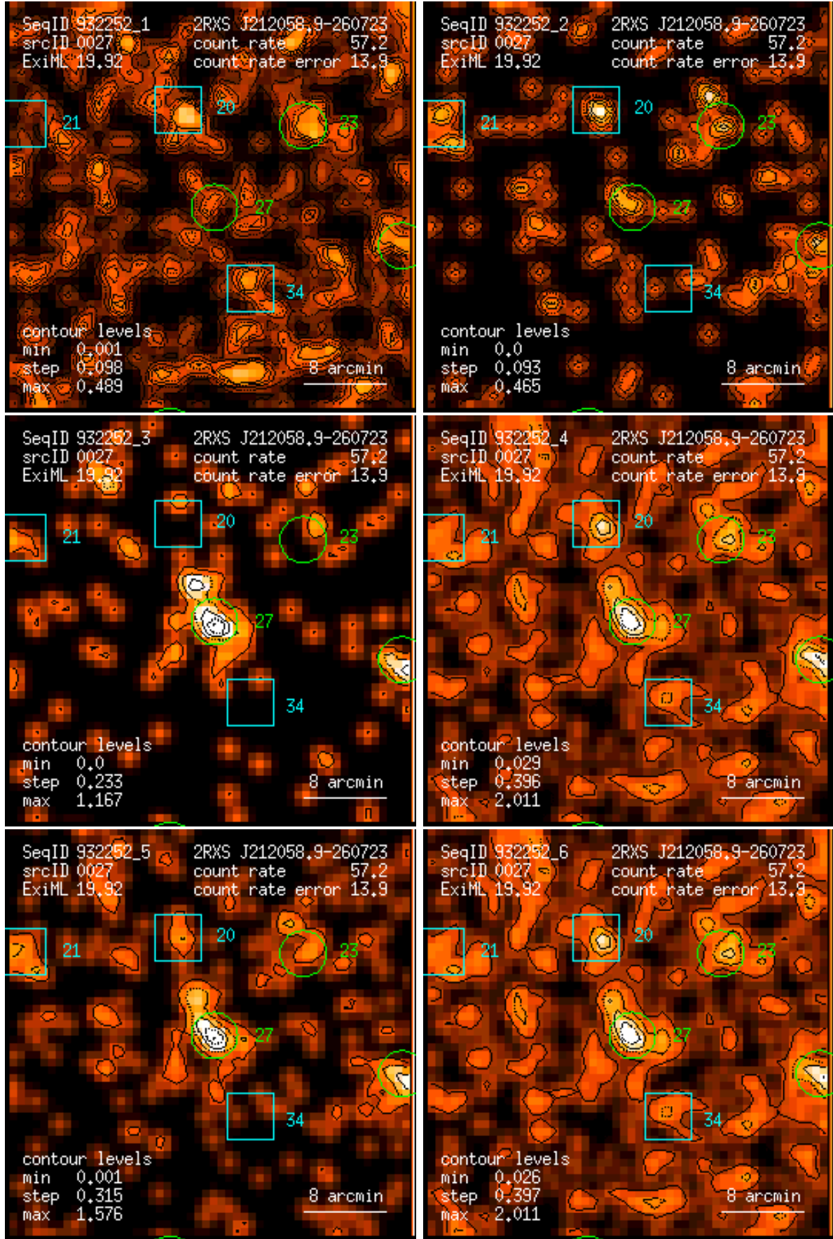
Figure 27: RASS 932252: detection 0027: band rate images, Gaussian filter: (1) PSPC channels 11 – 41, (2) 52 – 90, (3) 91 – 201, (4) 11 – 235, (5) 52 – 201, (6) 11 – 201. Broad band rates in counts/ks. Band rate contour levels in counts/ks/arcmin 2 .
