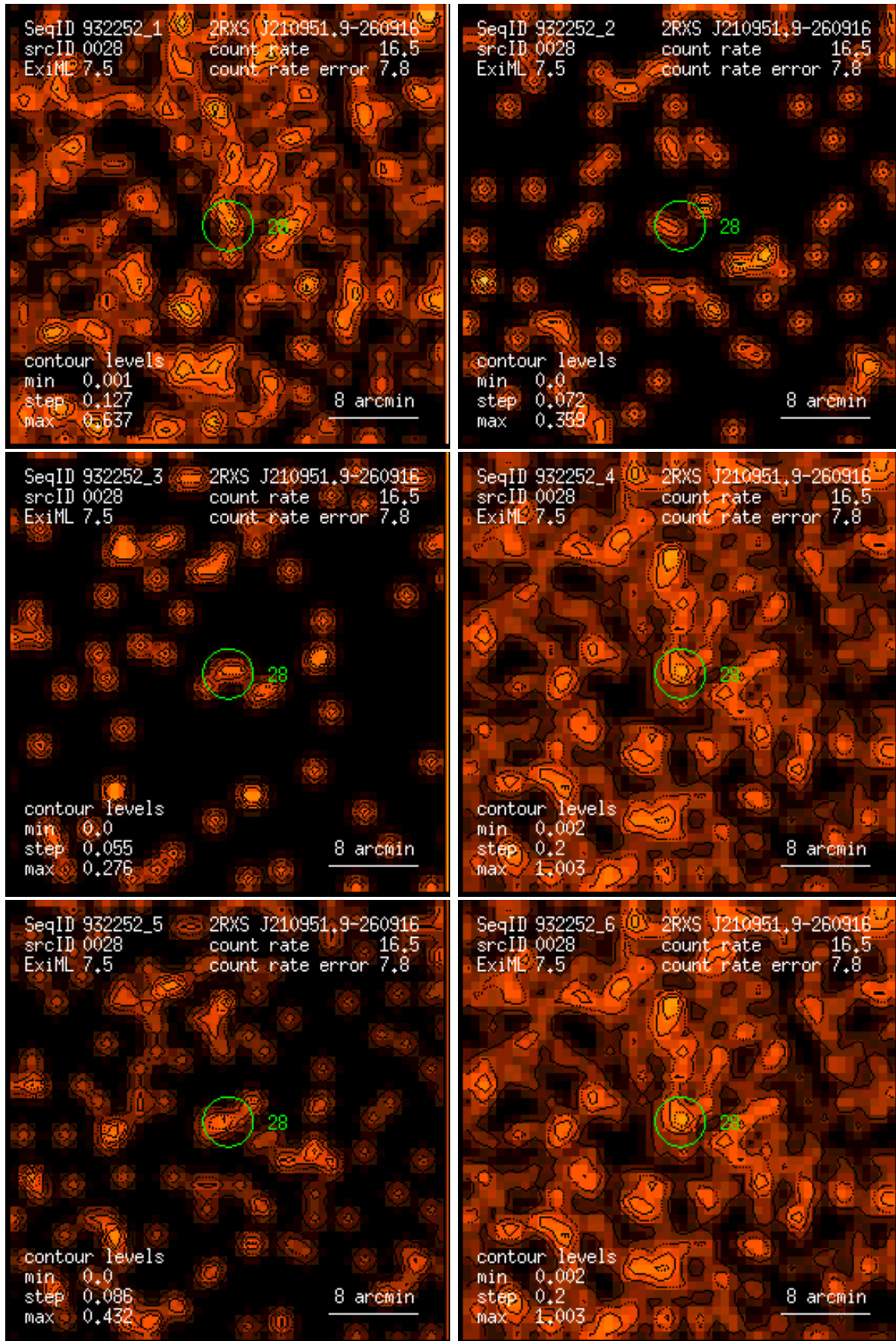
Figure 28: RASS 932252: detection 0028: band rate images, Gaussian filter: (1) PSPC channels 11 – 41, (2) 52 – 90, (3) 91 – 201, (4) 11 – 235, (5) 52 – 201, (6) 11 – 201. Broad band rates in counts/ks. Band rate contour levels in counts/ks/arcmin 2 .
