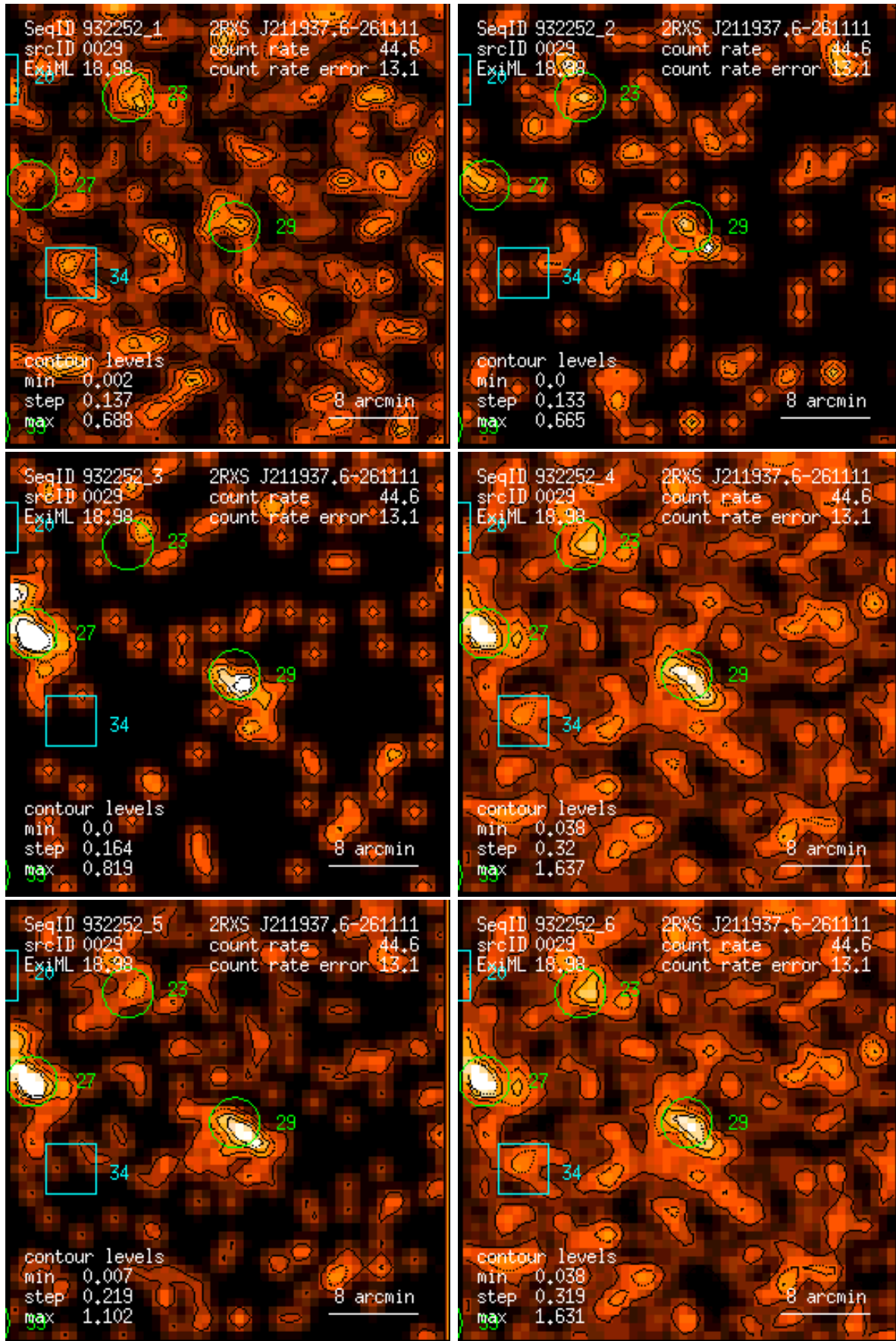
Figure 29: RASS 932252: detection 0029: band rate images, Gaussian filter: (1) PSPC channels 11 – 41, (2) 52 – 90, (3) 91 – 201, (4) 11 – 235, (5) 52 – 201, (6) 11 – 201. Broad band rates in counts/ks. Band rate contour levels in counts/ks/arcmin 2 .
