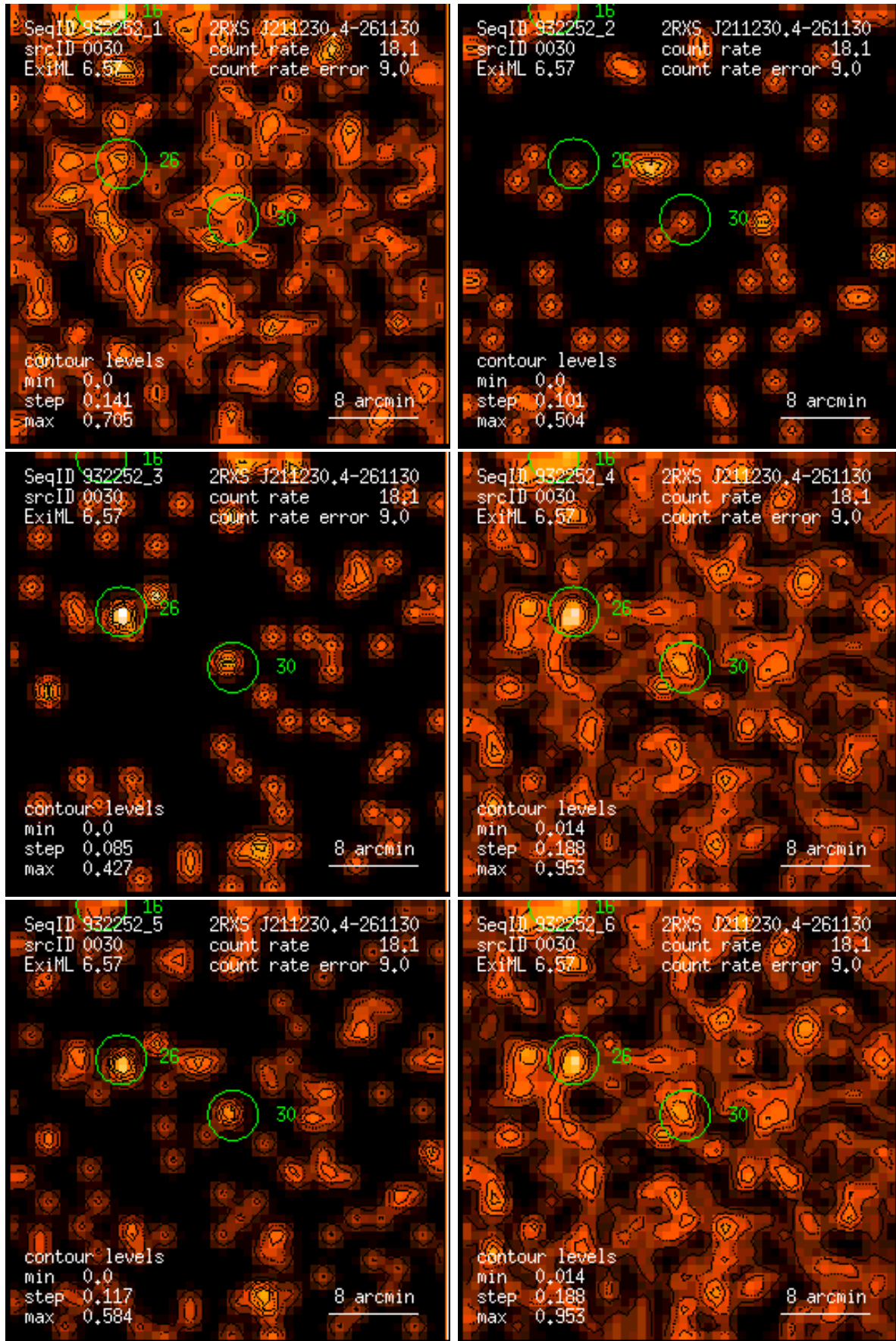
Figure 30: RASS 932252: detection 0030: band rate images, Gaussian filter: (1) PSPC channels 11 – 41, (2) 52 – 90, (3) 91 – 201, (4) 11 – 235, (5) 52 – 201, (6) 11 – 201. Broad band rates in counts/ks. Band rate contour levels in counts/ks/arcmin 2 .
