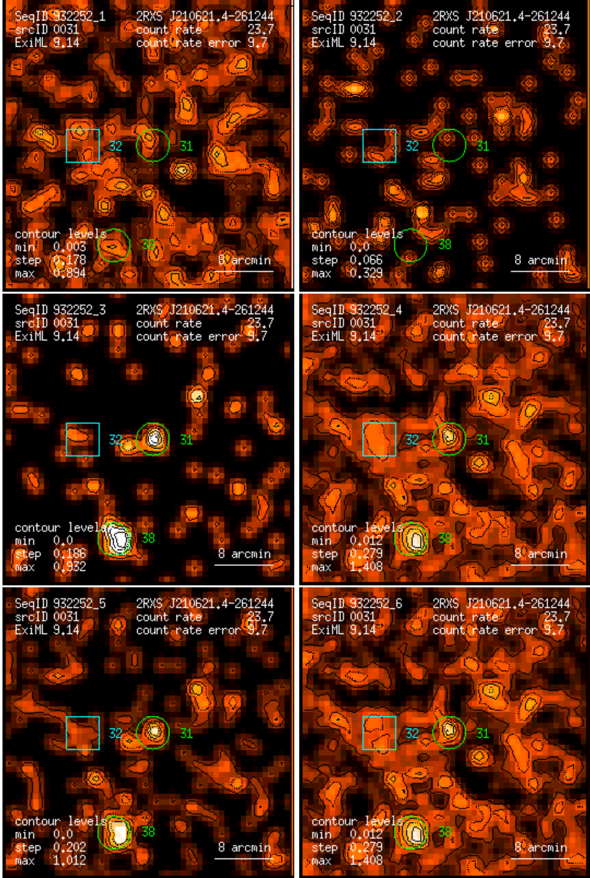
Figure 31: RASS 932252: detection 0031: band rate images, Gaussian filter: (1) PSPC channels 11 – 41, (2) 52 – 90, (3) 91 – 201, (4) 11 – 235, (5) 52 – 201, (6) 11 – 201. Broad band rates in counts/ks. Band rate contour levels in counts/ks/arcmin 2 .
