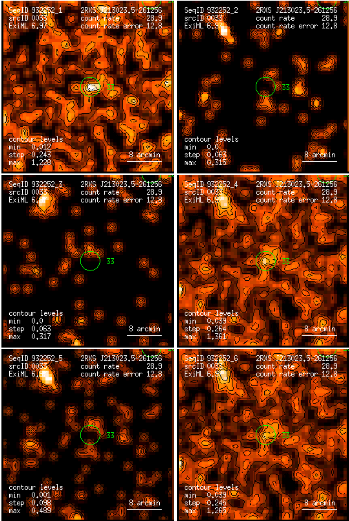
Figure 33: RASS 932252: detection 0033: band rate images, Gaussian filter: (1) PSPC channels 11 – 41, (2) 52 – 90, (3) 91 – 201, (4) 11 – 235, (5) 52 – 201, (6) 11 – 201. Broad band rates in counts/ks. Band rate contour levels in counts/ks/arcmin 2 .
