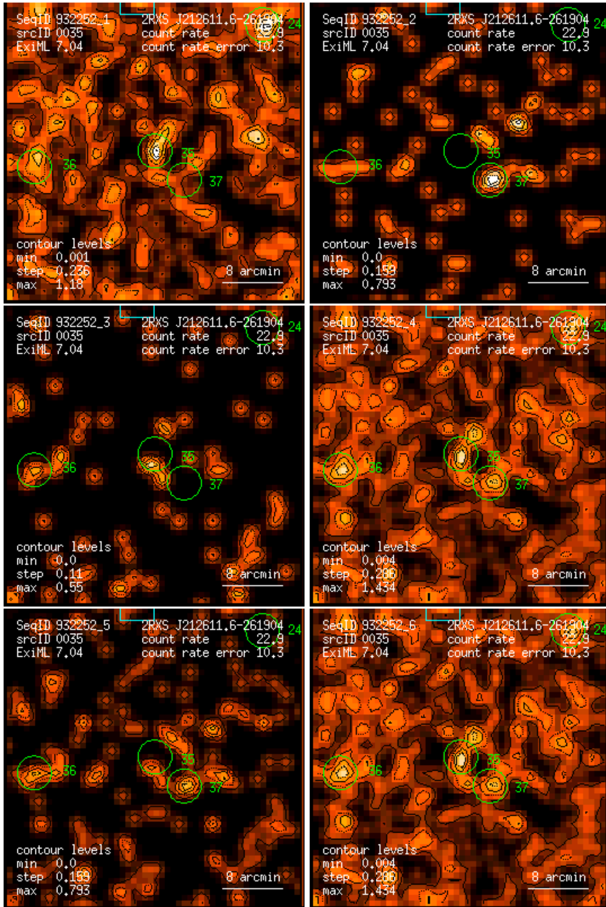
Figure 35: RASS 932252: detection 0035: band rate images, Gaussian filter: (1) PSPC channels 11 – 41, (2) 52 – 90, (3) 91 – 201, (4) 11 – 235, (5) 52 – 201, (6) 11 – 201. Broad band rates in counts/ks. Band rate contour levels in counts/ks/arcmin 2 .
