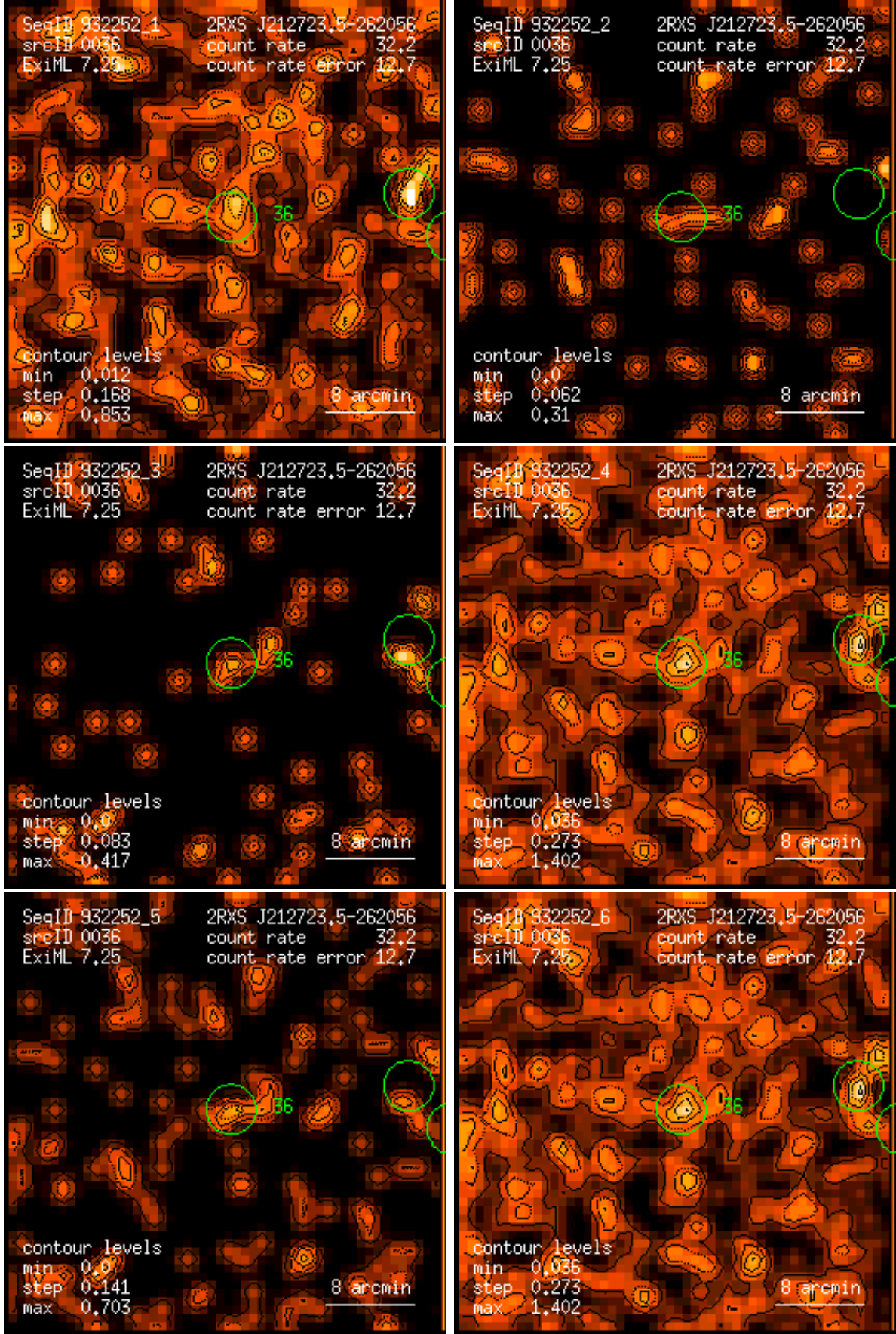
Figure 36: RASS 932252: detection 0036: band rate images, Gaussian filter: (1) PSPC channels 11 – 41, (2) 52 – 90, (3) 91 – 201, (4) 11 – 235, (5) 52 – 201, (6) 11 – 201. Broad band rates in counts/ks. Band rate contour levels in counts/ks/arcmin 2 .
