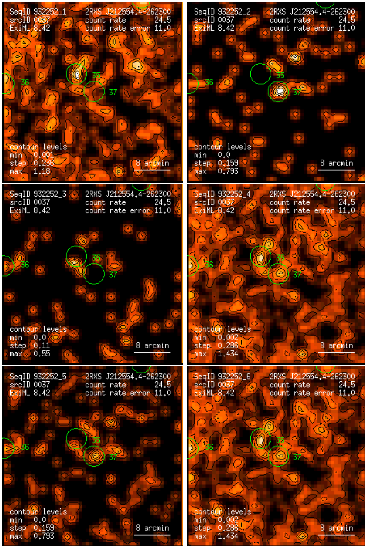
Figure 37: RASS 932252: detection 0037: band rate images, Gaussian filter: (1) PSPC channels 11 – 41, (2) 52 – 90, (3) 91 – 201, (4) 11 – 235, (5) 52 – 201, (6) 11 – 201. Broad band rates in counts/ks. Band rate contour levels in counts/ks/arcmin 2 .
