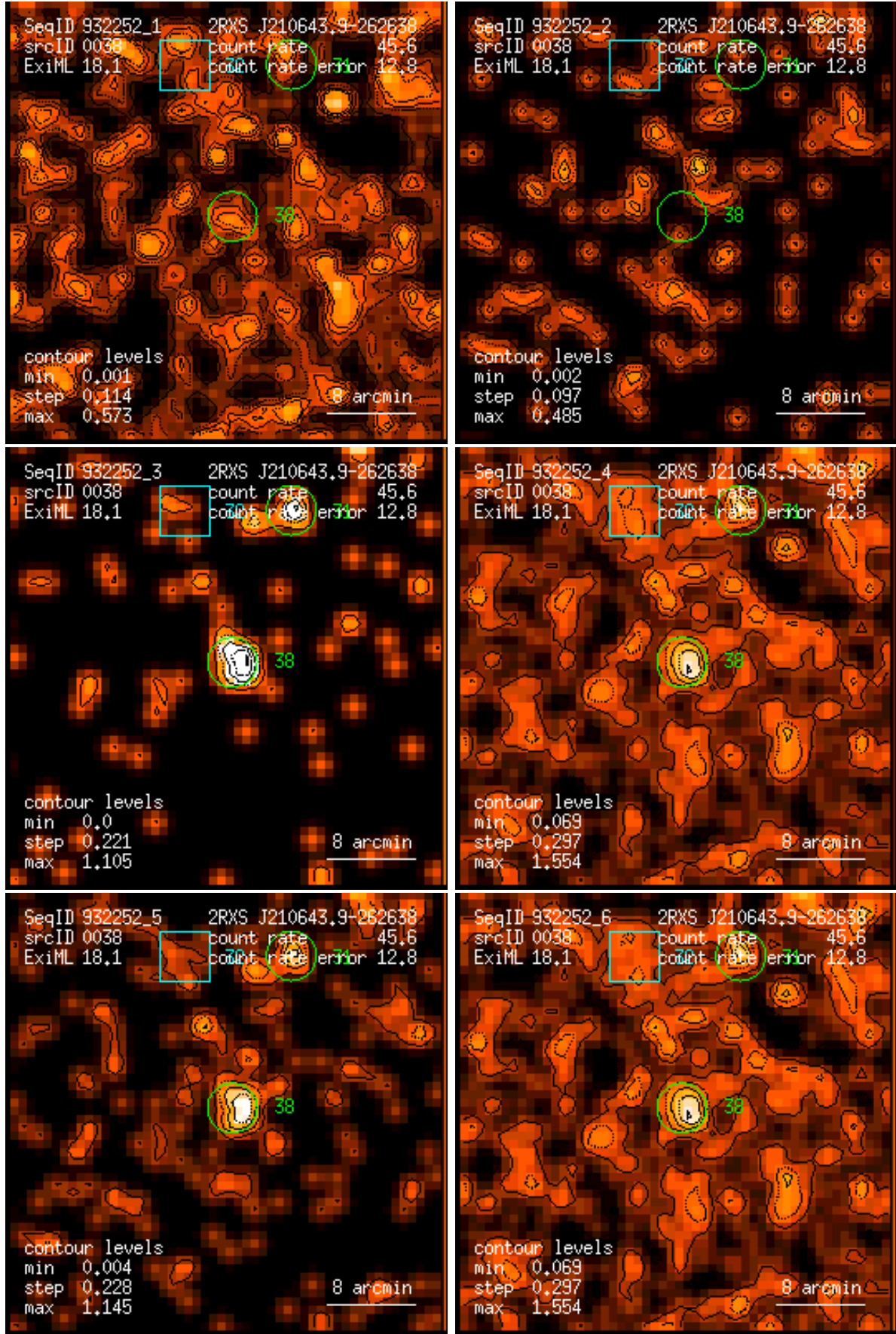
Figure 38: RASS 932252: detection 0038: band rate images, Gaussian filter: (1) PSPC channels 11 – 41, (2) 52 – 90, (3) 91 – 201, (4) 11 – 235, (5) 52 – 201, (6) 11 – 201. Broad band rates in counts/ks. Band rate contour levels in counts/ks/arcmin 2 .
