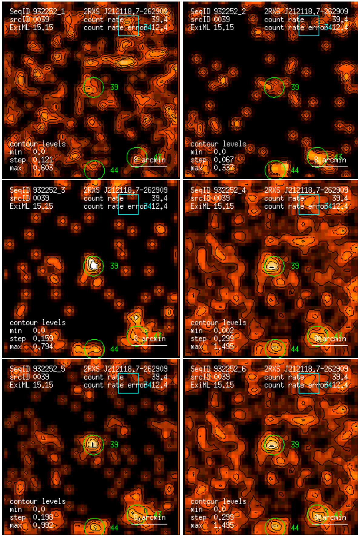
Figure 39: RASS 932252: detection 0039: band rate images, Gaussian filter: (1) PSPC channels 11 – 41, (2) 52 – 90, (3) 91 – 201, (4) 11 – 235, (5) 52 – 201, (6) 11 – 201. Broad band rates in counts/ks. Band rate contour levels in counts/ks/arcmin 2 .
