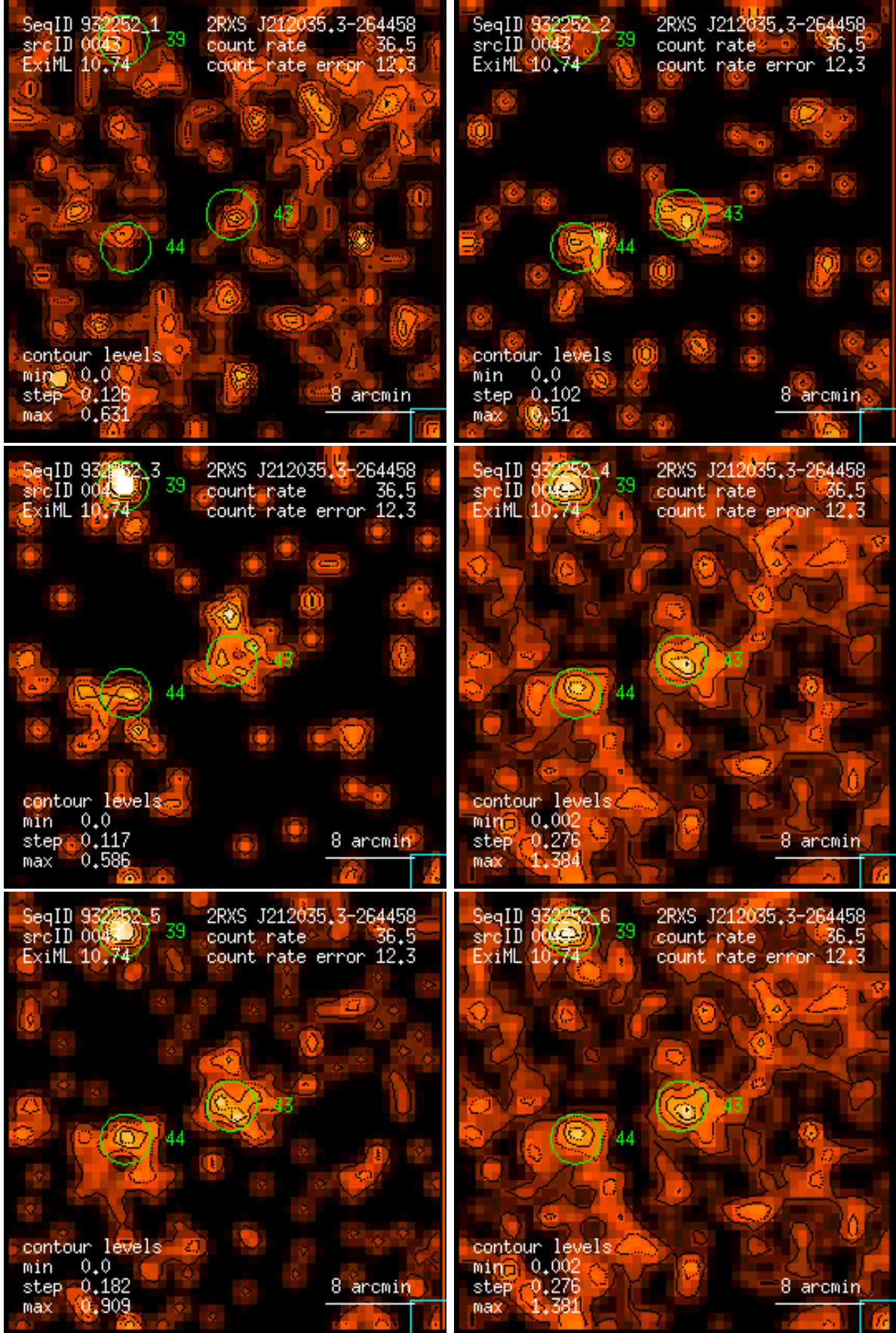
Figure 43: RASS 932252: detection 0043: band rate images, Gaussian filter: (1) PSPC channels 11 – 41, (2) 52 – 90, (3) 91 – 201, (4) 11 – 235, (5) 52 – 201, (6) 11 – 201. Broad band rates in counts/ks. Band rate contour levels in counts/ks/arcmin 2 .
