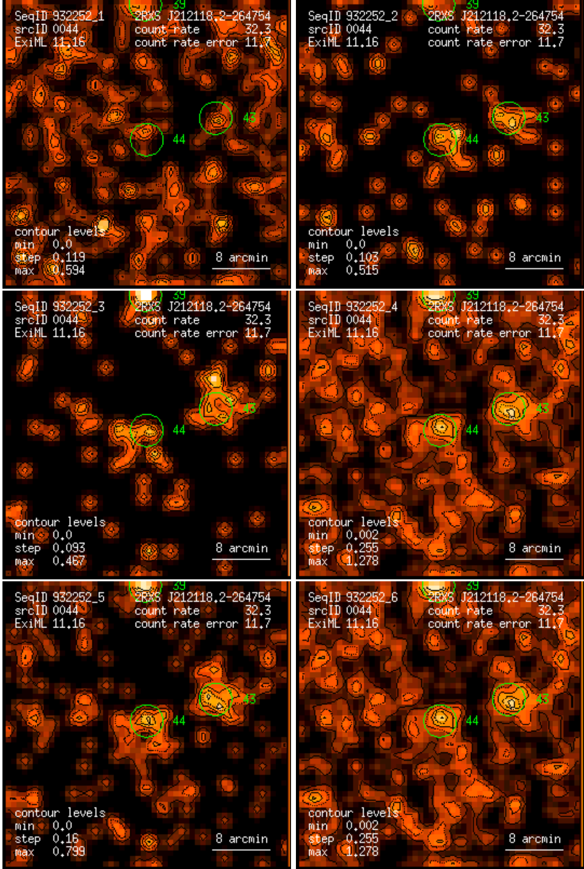
Figure 44: RASS 932252: detection 0044: band rate images, Gaussian filter: (1) PSPC channels 11 – 41, (2) 52 – 90, (3) 91 – 201, (4) 11 – 235, (5) 52 – 201, (6) 11 – 201. Broad band rates in counts/ks. Band rate contour levels in counts/ks/arcmin 2 .
