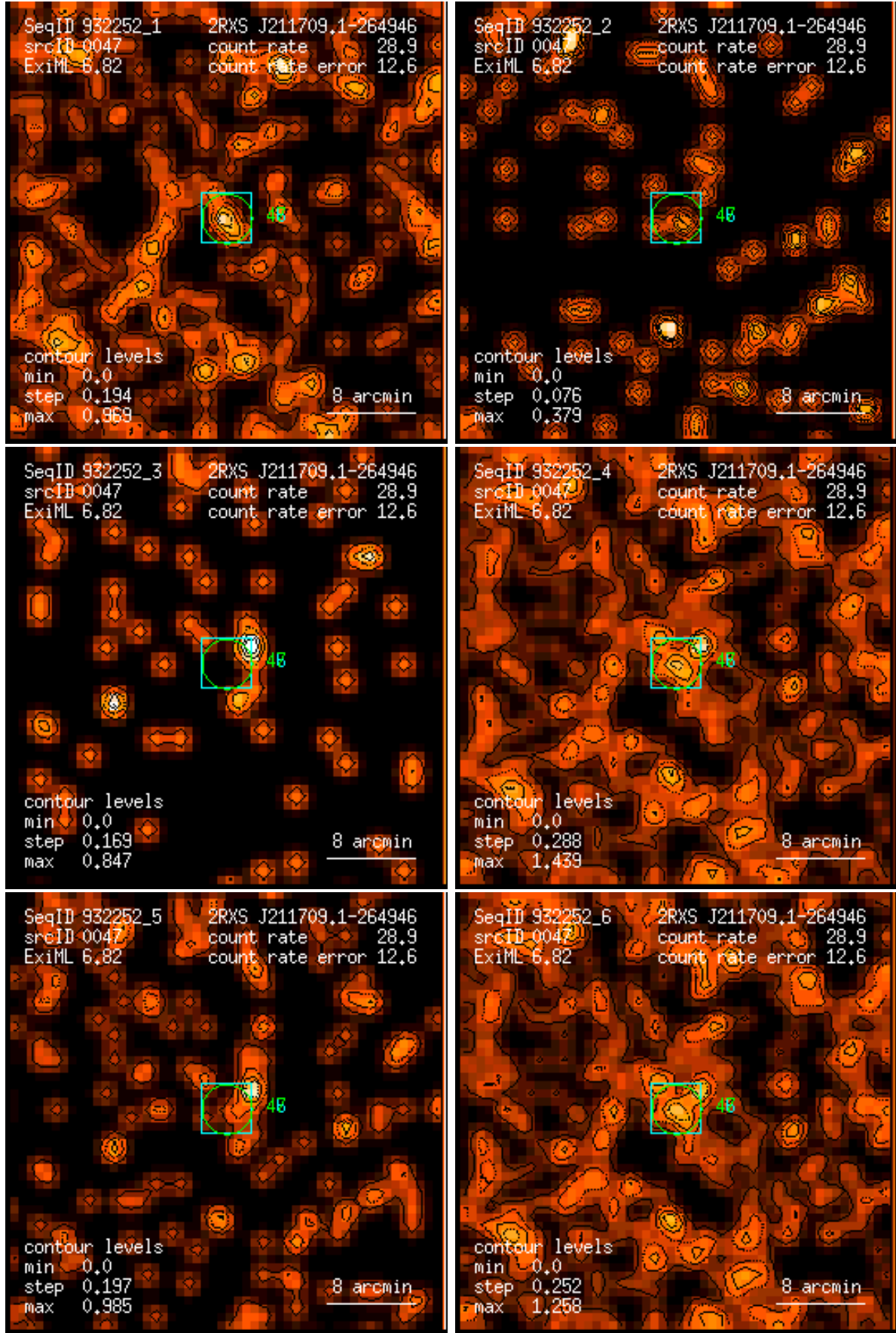
Figure 47: RASS 932252: detection 0047: band rate images, Gaussian filter: (1) PSPC channels 11 – 41, (2) 52 – 90, (3) 91 – 201, (4) 11 – 235, (5) 52 – 201, (6) 11 – 201. Broad band rates in counts/ks. Band rate contour levels in counts/ks/arcmin 2 .
