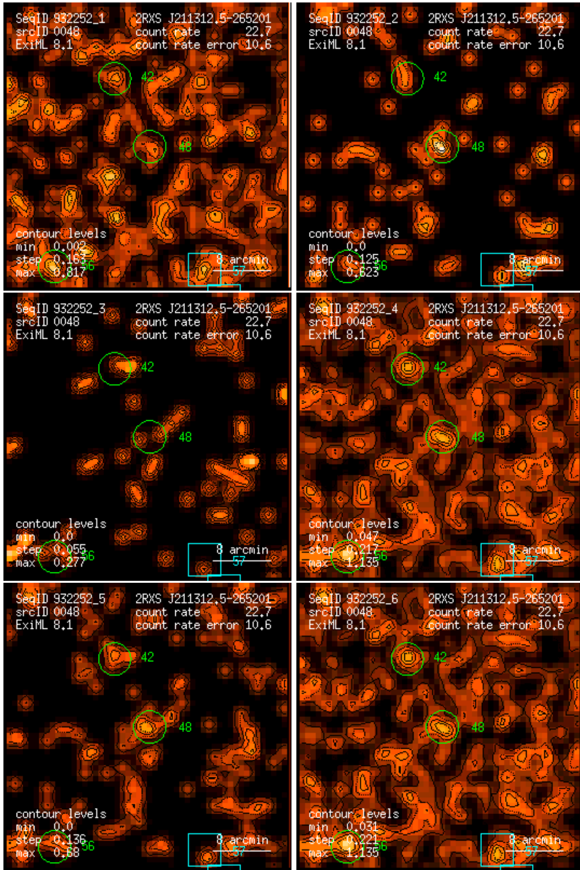
Figure 48: RASS 932252: detection 0048: band rate images, Gaussian filter: (1) PSPC channels 11 – 41, (2) 52 – 90, (3) 91 – 201, (4) 11 – 235, (5) 52 – 201, (6) 11 – 201. Broad band rates in counts/ks. Band rate contour levels in counts/ks/arcmin 2 .
