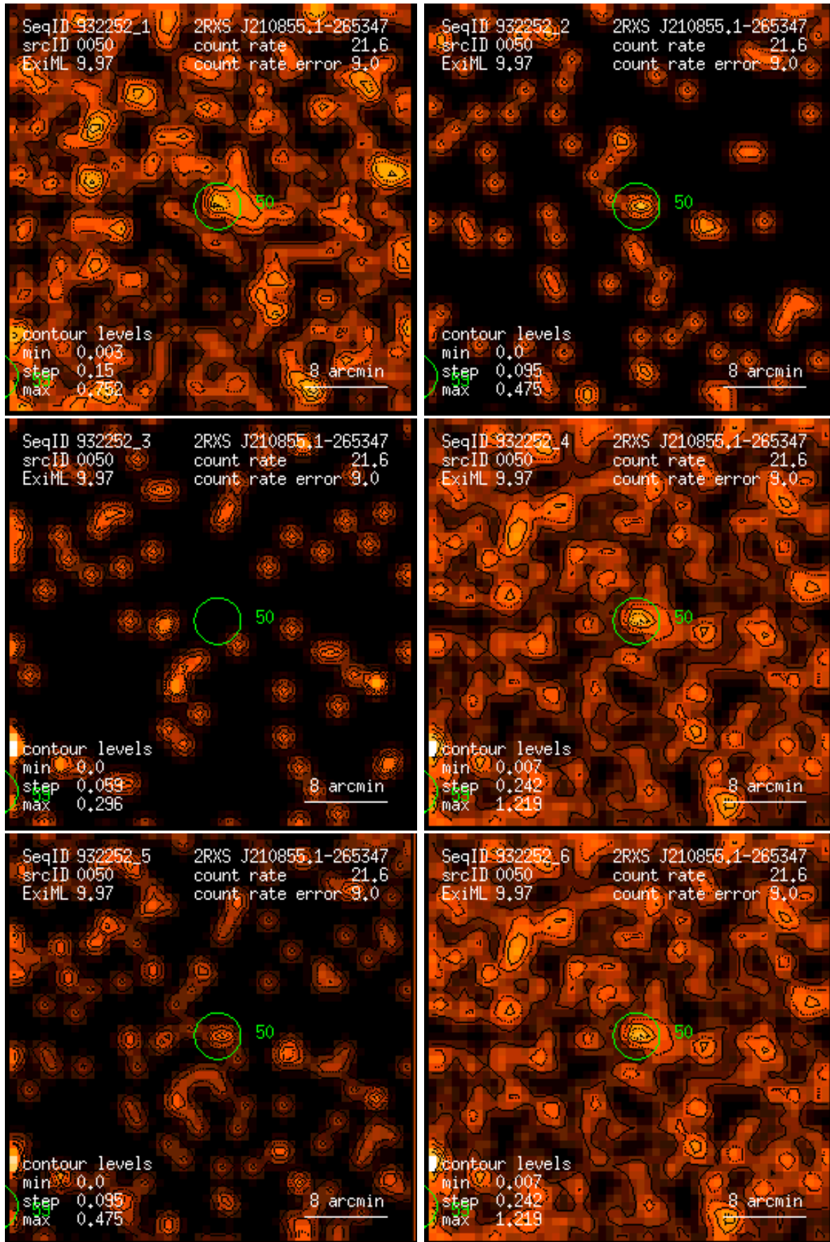
Figure 50: RASS 932252: detection 0050: band rate images, Gaussian filter: (1) PSPC channels 11 – 41, (2) 52 – 90, (3) 91 – 201, (4) 11 – 235, (5) 52 – 201, (6) 11 – 201. Broad band rates in counts/ks. Band rate contour levels in counts/ks/arcmin 2 .
