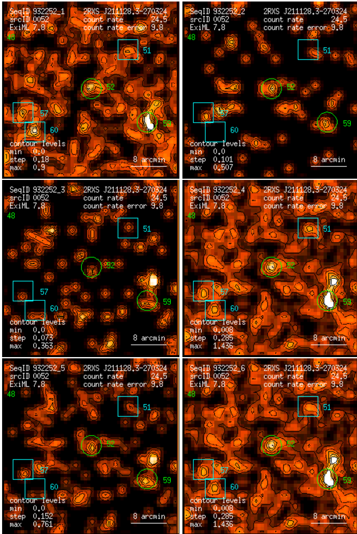
Figure 52: RASS 932252: detection 0052: band rate images, Gaussian filter: (1) PSPC channels 11 – 41, (2) 52 – 90, (3) 91 – 201, (4) 11 – 235, (5) 52 – 201, (6) 11 – 201. Broad band rates in counts/ks. Band rate contour levels in counts/ks/arcmin 2 .
