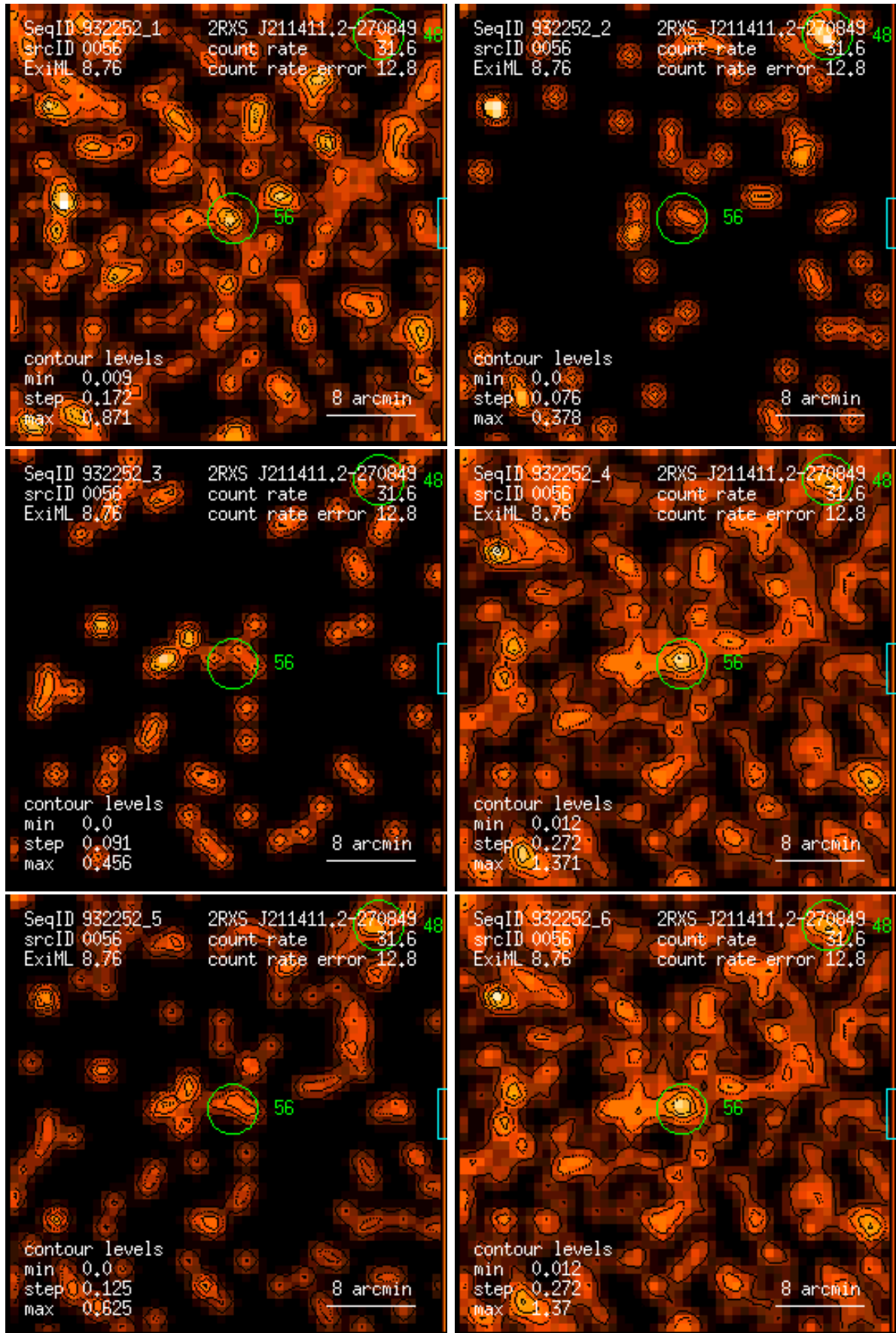
Figure 56: RASS 932252: detection 0056: band rate images, Gaussian filter: (1) PSPC channels 11 – 41, (2) 52 – 90, (3) 91 – 201, (4) 11 – 235, (5) 52 – 201, (6) 11 – 201. Broad band rates in counts/ks. Band rate contour levels in counts/ks/arcmin 2 .
