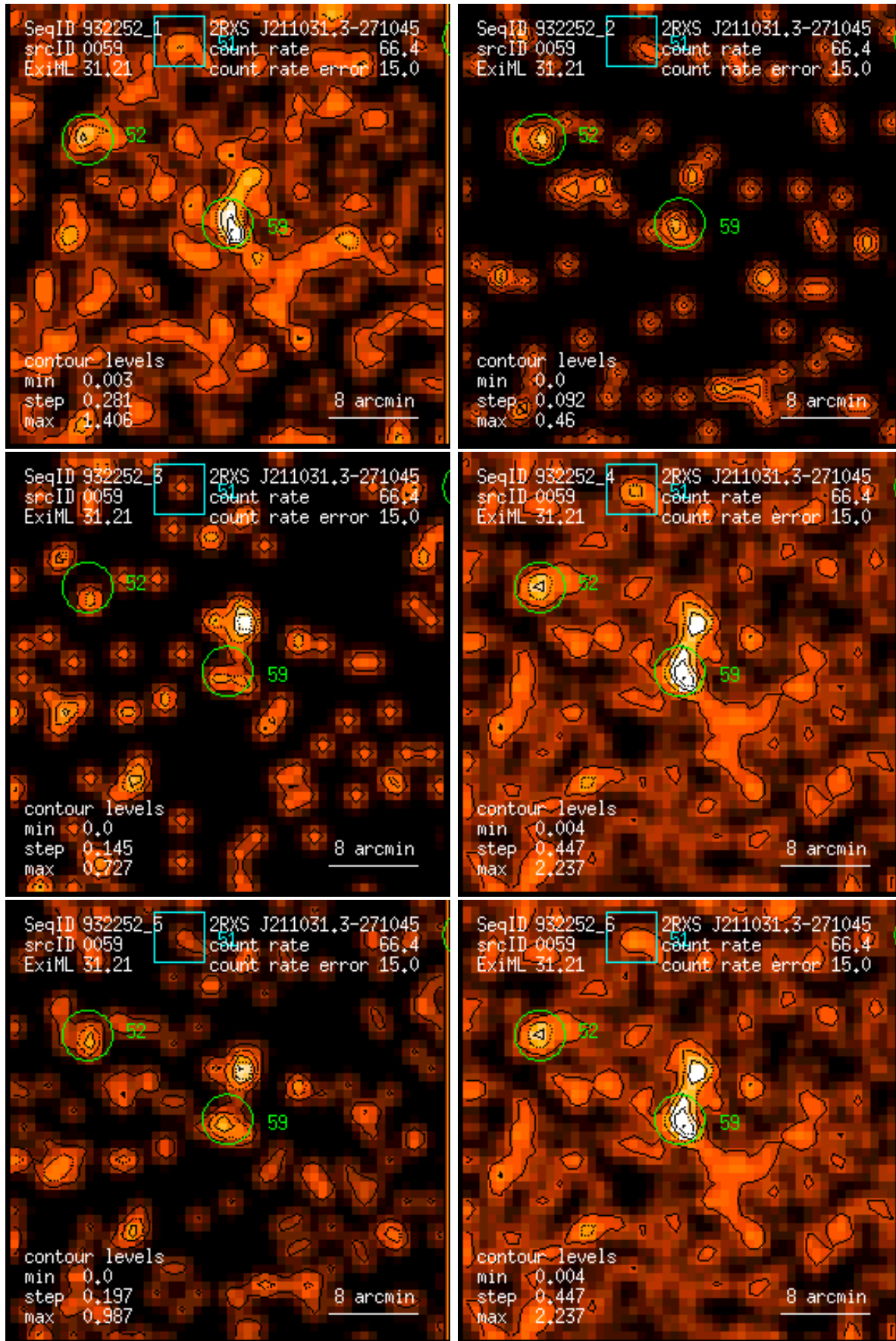
Figure 59: RASS 932252: detection 0059: band rate images, Gaussian filter: (1) PSPC channels 11 – 41, (2) 52 – 90, (3) 91 – 201, (4) 11 – 235, (5) 52 – 201, (6) 11 – 201. Broad band rates in counts/ks. Band rate contour levels in counts/ks/arcmin 2 .
