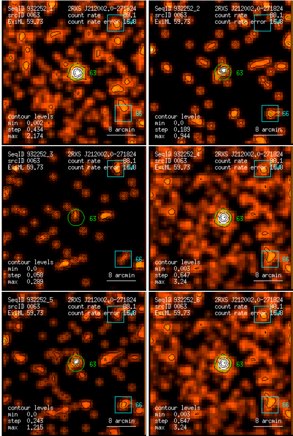
Figure 63: RASS 932252: detection 0063: band rate images, Gaussian filter: (1) PSPC channels 11 – 41, (2) 52 – 90, (3) 91 – 201, (4) 11 – 235, (5) 52 – 201, (6) 11 – 201. Broad band rates in counts/ks. Band rate contour levels in counts/ks/arcmin 2 .
