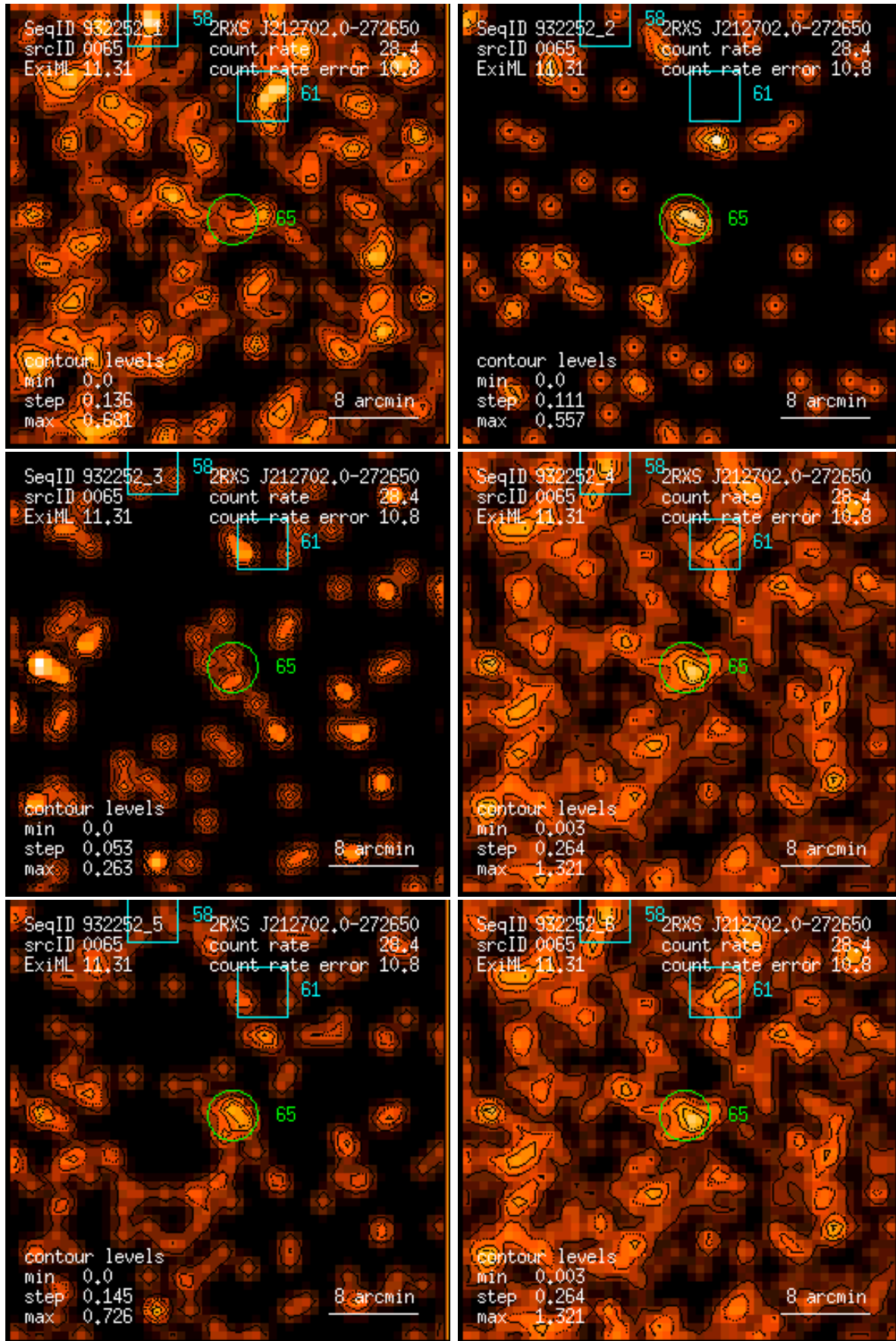
Figure 65: RASS 932252: detection 0065: band rate images, Gaussian filter: (1) PSPC channels 11 – 41, (2) 52 – 90, (3) 91 – 201, (4) 11 – 235, (5) 52 – 201, (6) 11 – 201. Broad band rates in counts/ks. Band rate contour levels in counts/ks/arcmin 2 .
