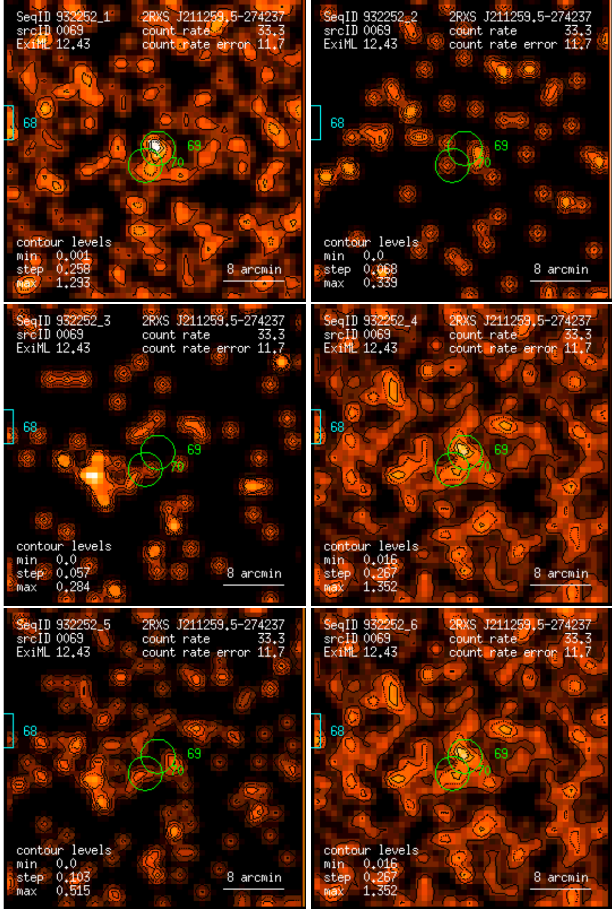
Figure 69: RASS 932252: detection 0069: band rate images, Gaussian filter: (1) PSPC channels 11 – 41, (2) 52 – 90, (3) 91 – 201, (4) 11 – 235, (5) 52 – 201, (6) 11 – 201. Broad band rates in counts/ks. Band rate contour levels in counts/ks/arcmin 2 .
