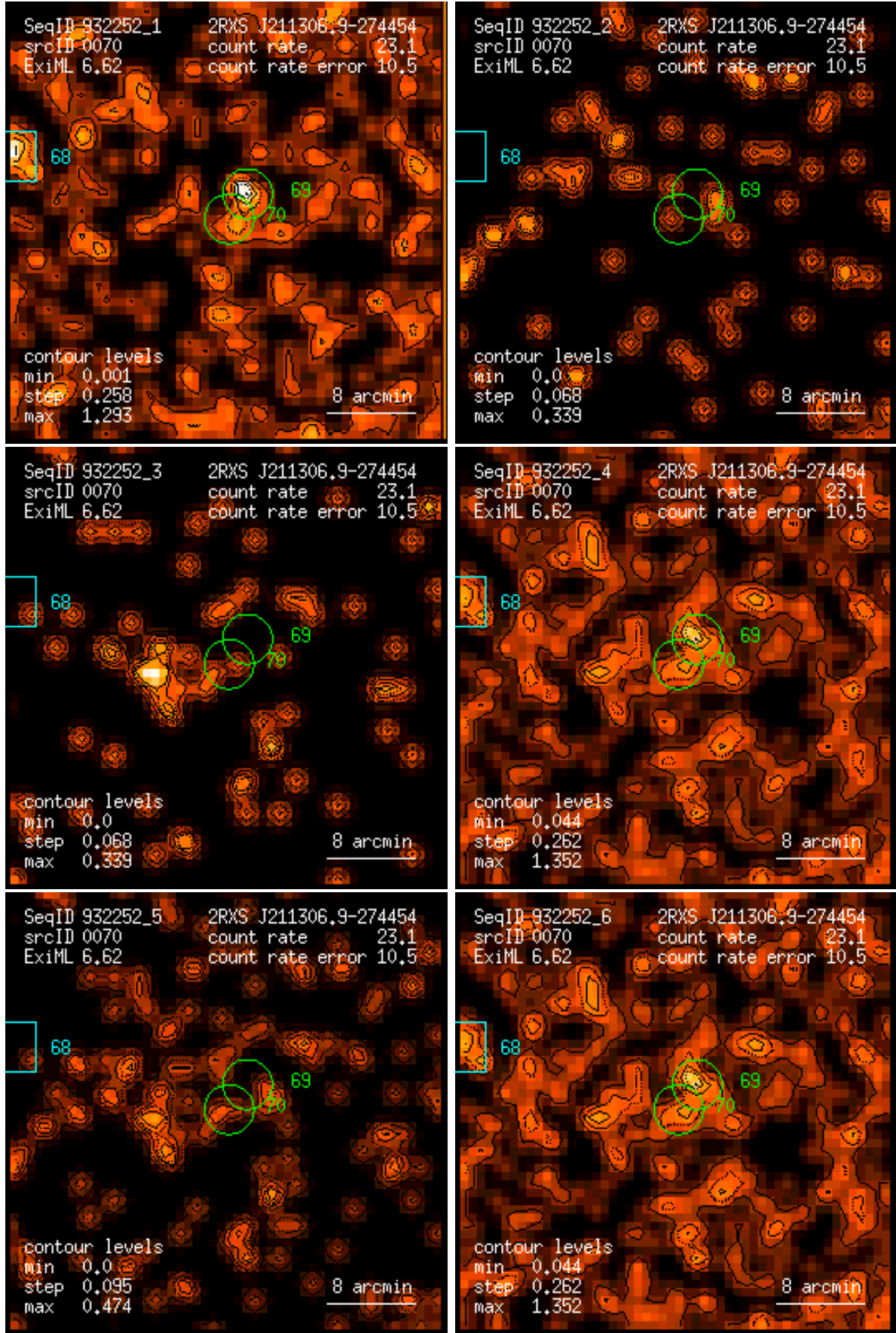
Figure 70: RASS 932252: detection 0070: band rate images, Gaussian filter: (1) PSPC channels 11 – 41, (2) 52 – 90, (3) 91 – 201, (4) 11 – 235, (5) 52 – 201, (6) 11 – 201. Broad band rates in counts/ks. Band rate contour levels in counts/ks/arcmin 2 .
