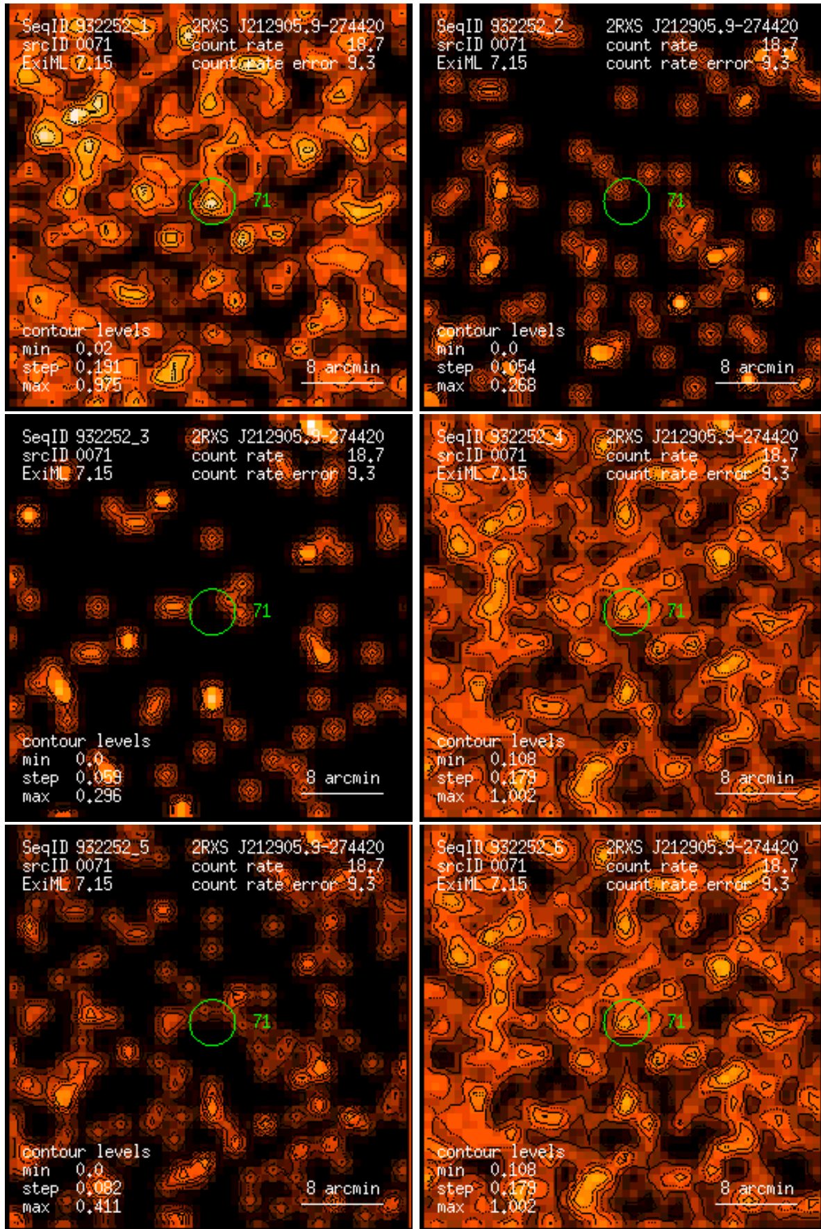
Figure 71: RASS 932252: detection 0071: band rate images, Gaussian filter: (1) PSPC channels 11 – 41, (2) 52 – 90, (3) 91 – 201, (4) 11 – 235, (5) 52 – 201, (6) 11 – 201. Broad band rates in counts/ks. Band rate contour levels in counts/ks/arcmin 2 .
