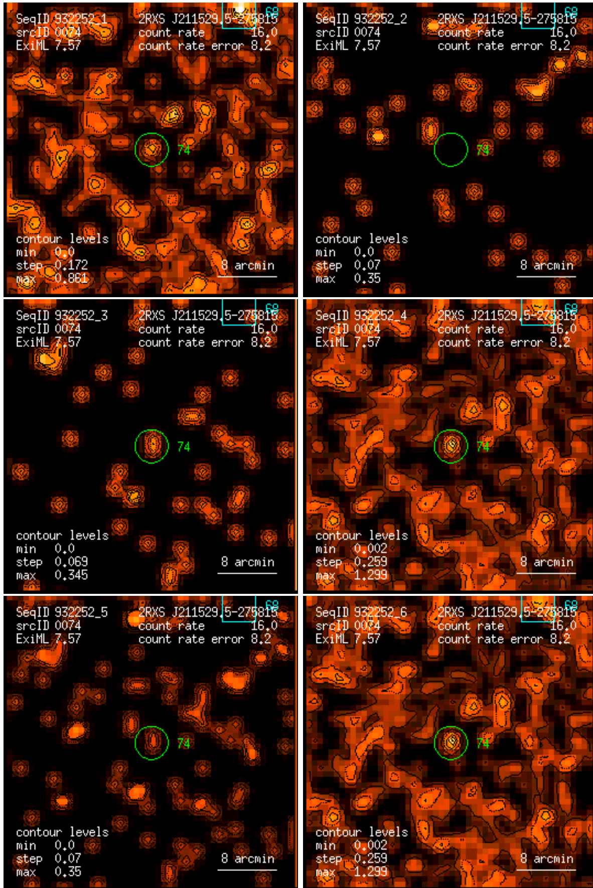
Figure 74: RASS 932252: detection 0074: band rate images, Gaussian filter: (1) PSPC channels 11 – 41, (2) 52 – 90, (3) 91 – 201, (4) 11 – 235, (5) 52 – 201, (6) 11 – 201. Broad band rates in counts/ks. Band rate contour levels in counts/ks/arcmin 2 .
