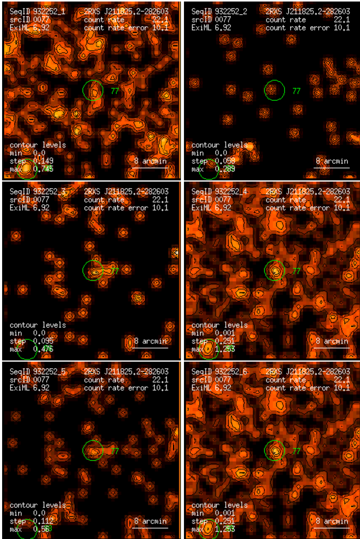
Figure 77: RASS 932252: detection 0077: band rate images, Gaussian filter: (1) PSPC channels 11 – 41, (2) 52 – 90, (3) 91 – 201, (4) 11 – 235, (5) 52 – 201, (6) 11 – 201. Broad band rates in counts/ks. Band rate contour levels in counts/ks/arcmin 2 .
