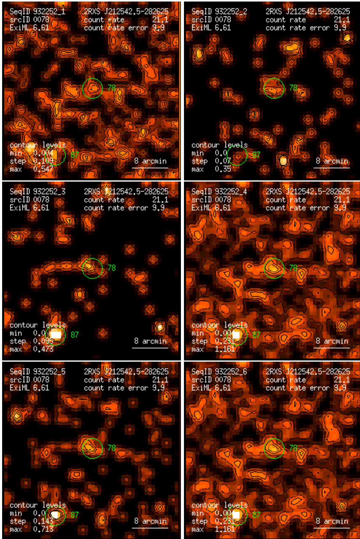
Figure 78: RASS 932252: detection 0078: band rate images, Gaussian filter: (1) PSPC channels 11 – 41, (2) 52 – 90, (3) 91 – 201, (4) 11 – 235, (5) 52 – 201, (6) 11 – 201. Broad band rates in counts/ks. Band rate contour levels in counts/ks/arcmin 2 .
