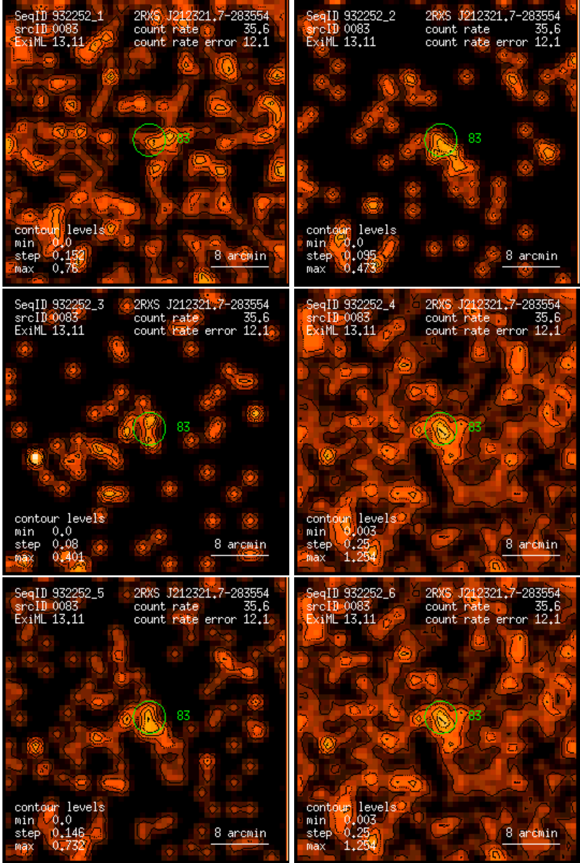
Figure 83: RASS 932252: detection 0083: band rate images, Gaussian filter: (1) PSPC channels 11 – 41, (2) 52 – 90, (3) 91 – 201, (4) 11 – 235, (5) 52 – 201, (6) 11 – 201. Broad band rates in counts/ks. Band rate contour levels in counts/ks/arcmin 2 .
