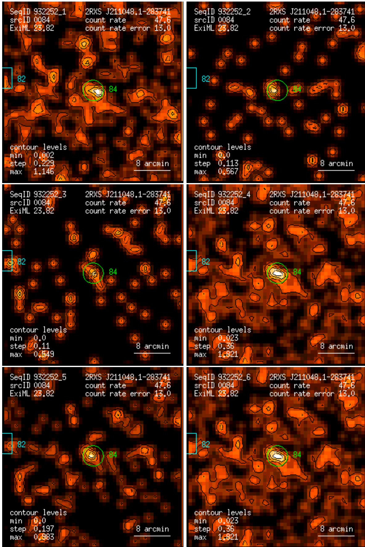
Figure 84: RASS 932252: detection 0084: band rate images, Gaussian filter: (1) PSPC channels 11 – 41, (2) 52 – 90, (3) 91 – 201, (4) 11 – 235, (5) 52 – 201, (6) 11 – 201. Broad band rates in counts/ks. Band rate contour levels in counts/ks/arcmin 2 .
