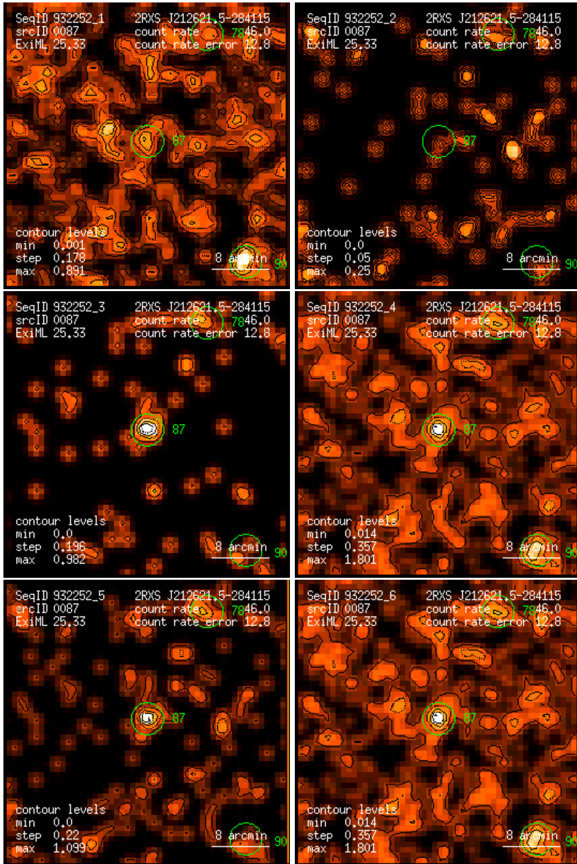
Figure 87: RASS 932252: detection 0087: band rate images, Gaussian filter: (1) PSPC channels 11 – 41, (2) 52 – 90, (3) 91 – 201, (4) 11 – 235, (5) 52 – 201, (6) 11 – 201. Broad band rates in counts/ks. Band rate contour levels in counts/ks/arcmin 2 .
