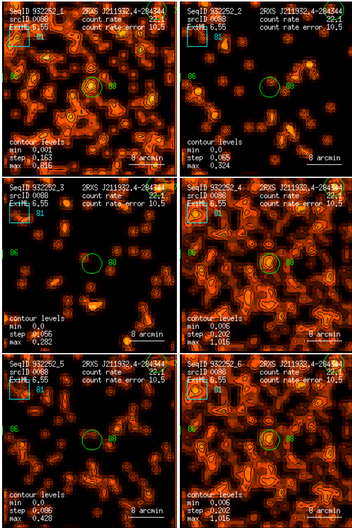
Figure 88: RASS 932252: detection 0088: band rate images, Gaussian filter: (1) PSPC channels 11 – 41, (2) 52 – 90, (3) 91 – 201, (4) 11 – 235, (5) 52 – 201, (6) 11 – 201. Broad band rates in counts/ks. Band rate contour levels in counts/ks/arcmin 2 .
