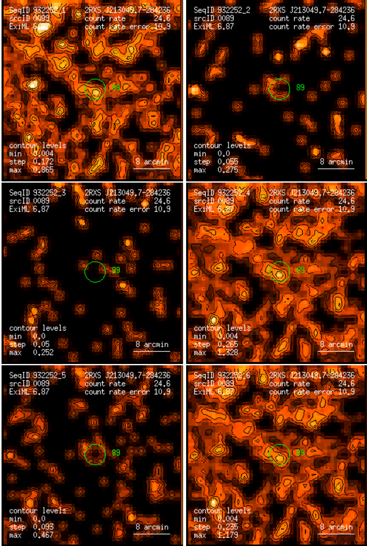
Figure 89: RASS 932252: detection 0089: band rate images, Gaussian filter: (1) PSPC channels 11 – 41, (2) 52 – 90, (3) 91 – 201, (4) 11 – 235, (5) 52 – 201, (6) 11 – 201. Broad band rates in counts/ks. Band rate contour levels in counts/ks/arcmin 2 .
