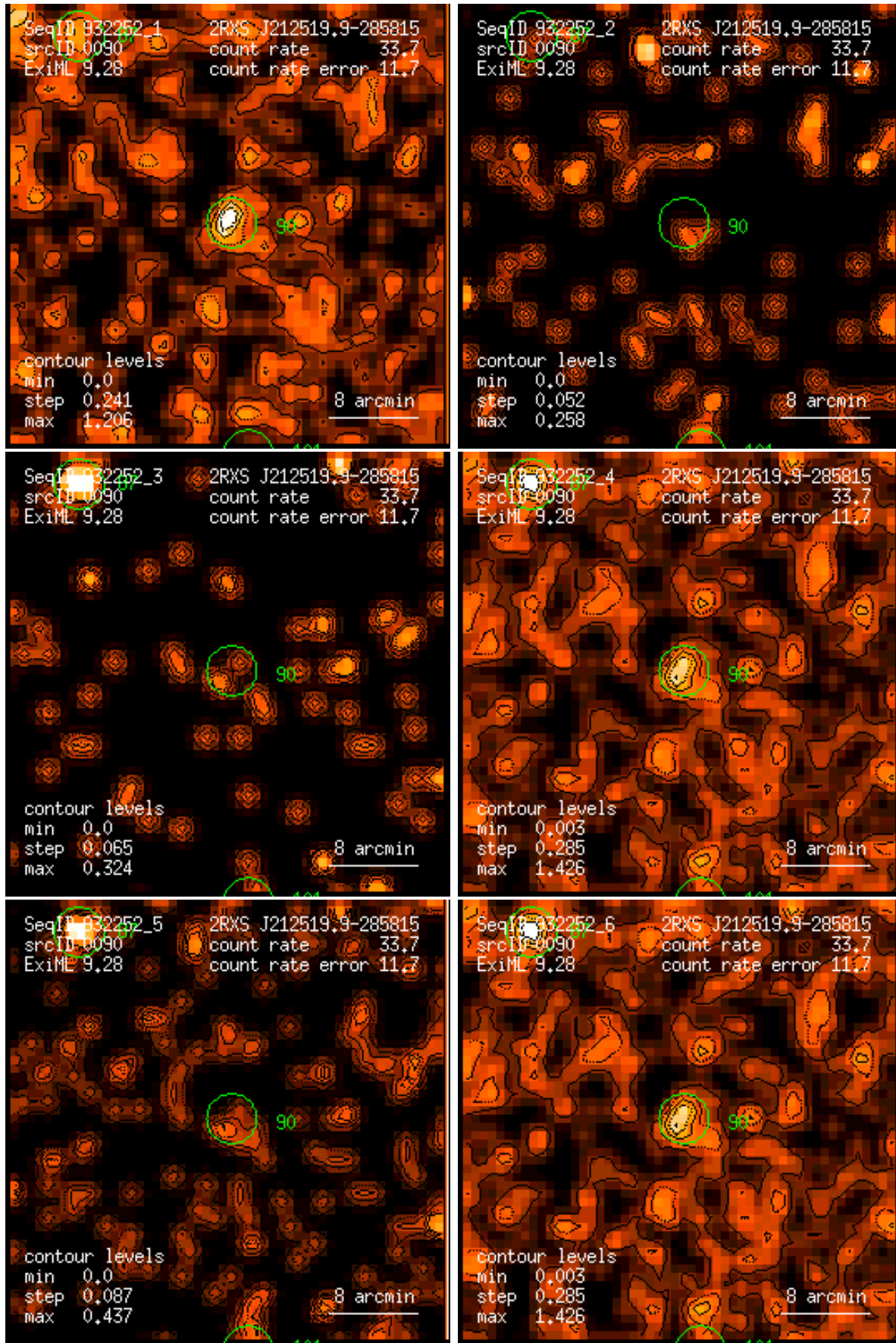
Figure 90: RASS 932252: detection 0090: band rate images, Gaussian filter: (1) PSPC channels 11 – 41, (2) 52 – 90, (3) 91 – 201, (4) 11 – 235, (5) 52 – 201, (6) 11 – 201. Broad band rates in counts/ks. Band rate contour levels in counts/ks/arcmin 2 .
