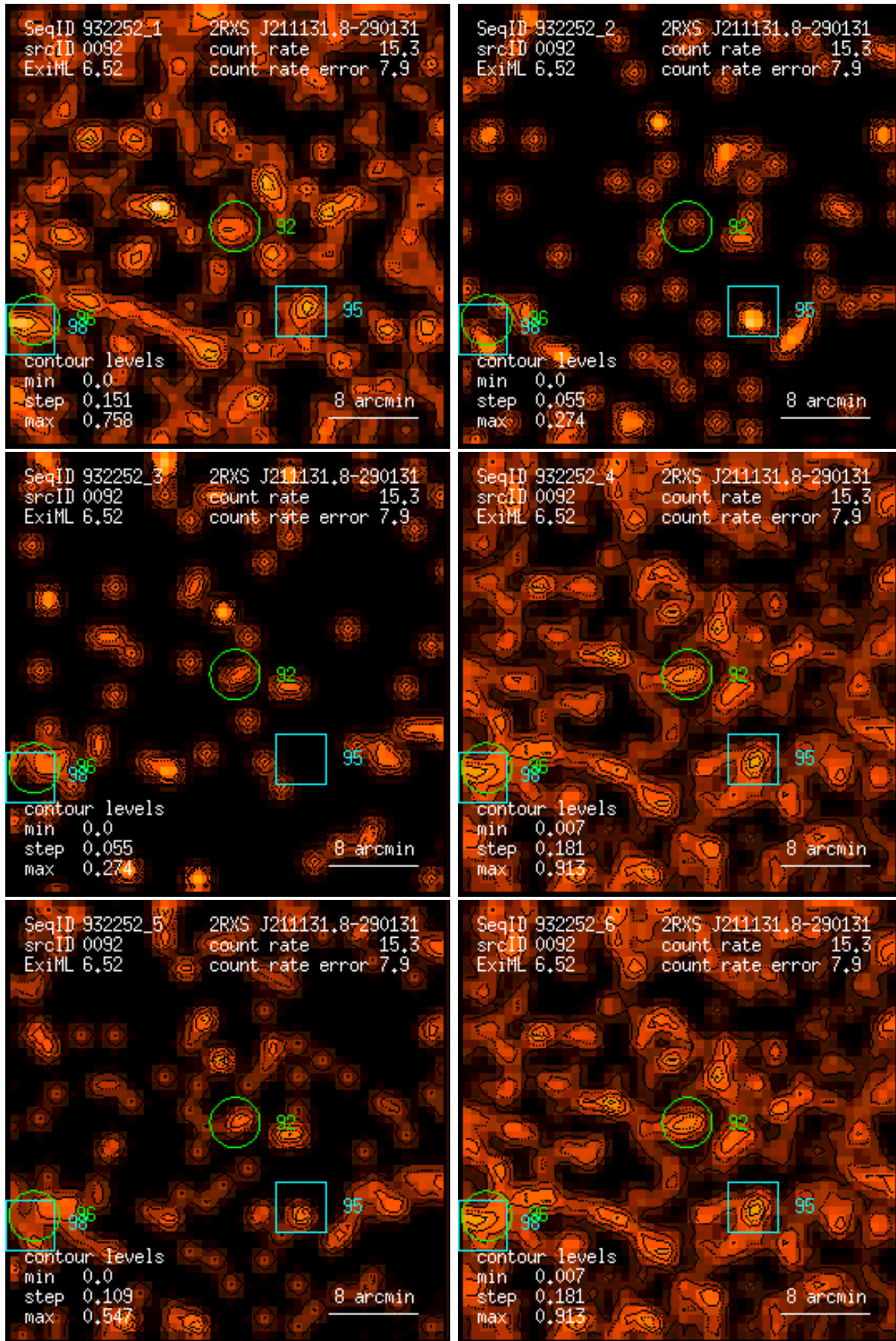
Figure 92: RASS 932252: detection 0092: band rate images, Gaussian filter: (1) PSPC channels 11 – 41, (2) 52 – 90, (3) 91 – 201, (4) 11 – 235, (5) 52 – 201, (6) 11 – 201. Broad band rates in counts/ks. Band rate contour levels in counts/ks/arcmin 2 .
