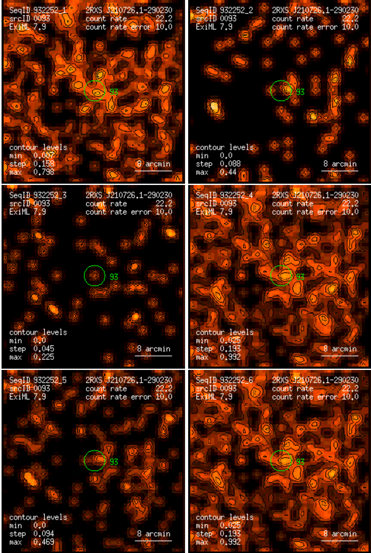
Figure 93: RASS 932252: detection 0093: band rate images, Gaussian filter: (1) PSPC channels 11 – 41, (2) 52 – 90, (3) 91 – 201, (4) 11 – 235, (5) 52 – 201, (6) 11 – 201. Broad band rates in counts/ks. Band rate contour levels in counts/ks/arcmin 2 .
