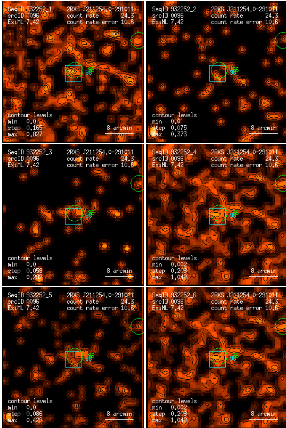
Figure 96: RASS 932252: detection 0096: band rate images, Gaussian filter: (1) PSPC channels 11 – 41, (2) 52 – 90, (3) 91 – 201, (4) 11 – 235, (5) 52 – 201, (6) 11 – 201. Broad band rates in counts/ks. Band rate contour levels in counts/ks/arcmin 2 .
