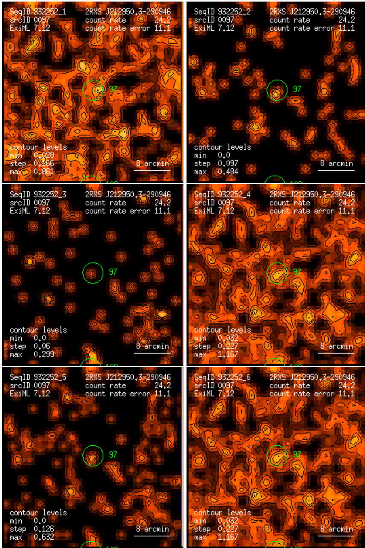
Figure 97: RASS 932252: detection 0097: band rate images, Gaussian filter: (1) PSPC channels 11 – 41, (2) 52 – 90, (3) 91 – 201, (4) 11 – 235, (5) 52 – 201, (6) 11 – 201. Broad band rates in counts/ks. Band rate contour levels in counts/ks/arcmin 2 .
