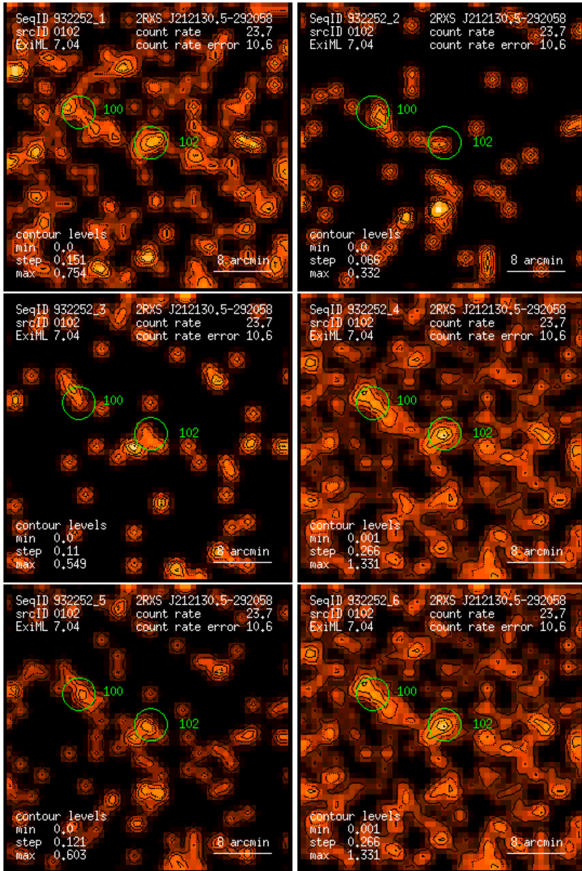
Figure 102: RASS 932252: detection 0102: band rate images, Gaussian filter: (1) PSPC channels 11 – 41, (2) 52 – 90, (3) 91 – 201, (4) 11 – 235, (5) 52 – 201, (6) 11 – 201. Broad band rates in counts/ks. Band rate contour levels in counts/ks/arcmin 2 .
