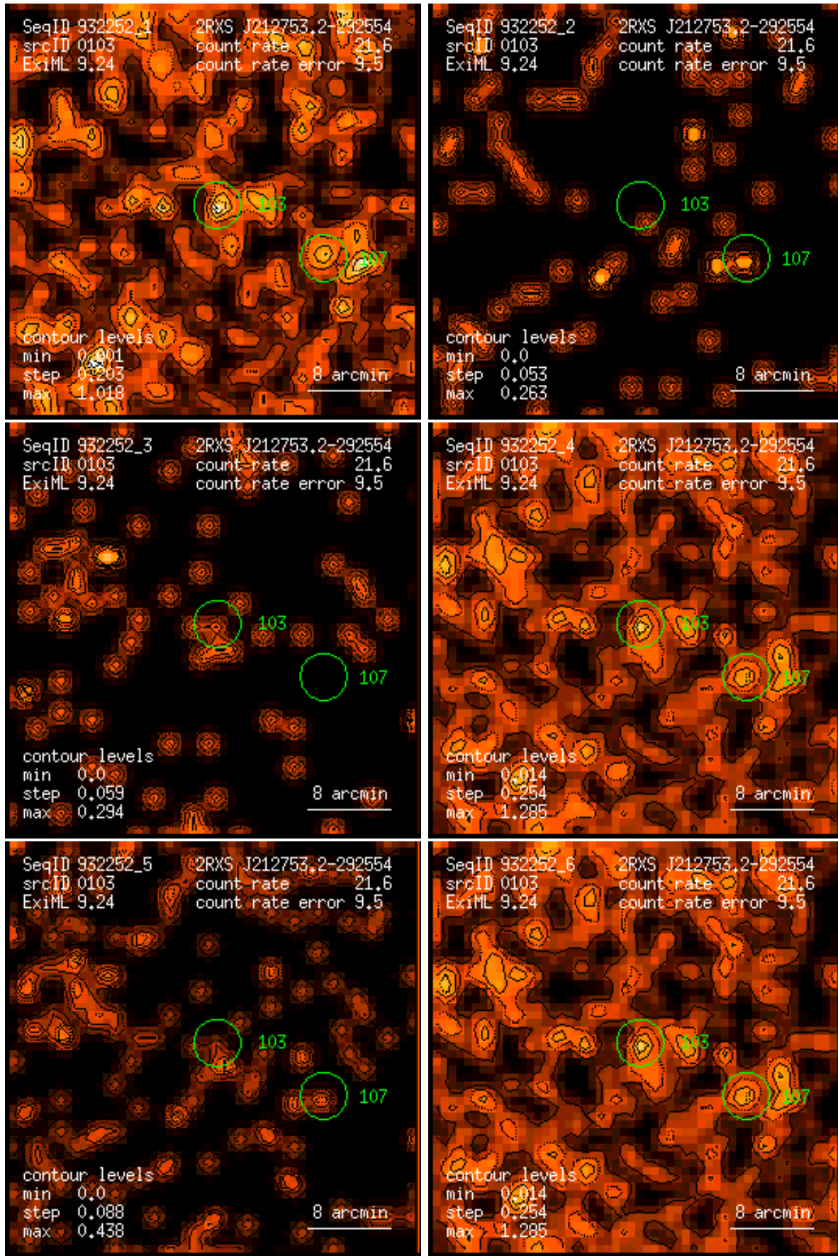
Figure 103: RASS 932252: detection 0103: band rate images, Gaussian filter: (1) PSPC channels 11 – 41, (2) 52 – 90, (3) 91 – 201, (4) 11 – 235, (5) 52 – 201, (6) 11 – 201. Broad band rates in counts/ks. Band rate contour levels in counts/ks/arcmin 2 .
