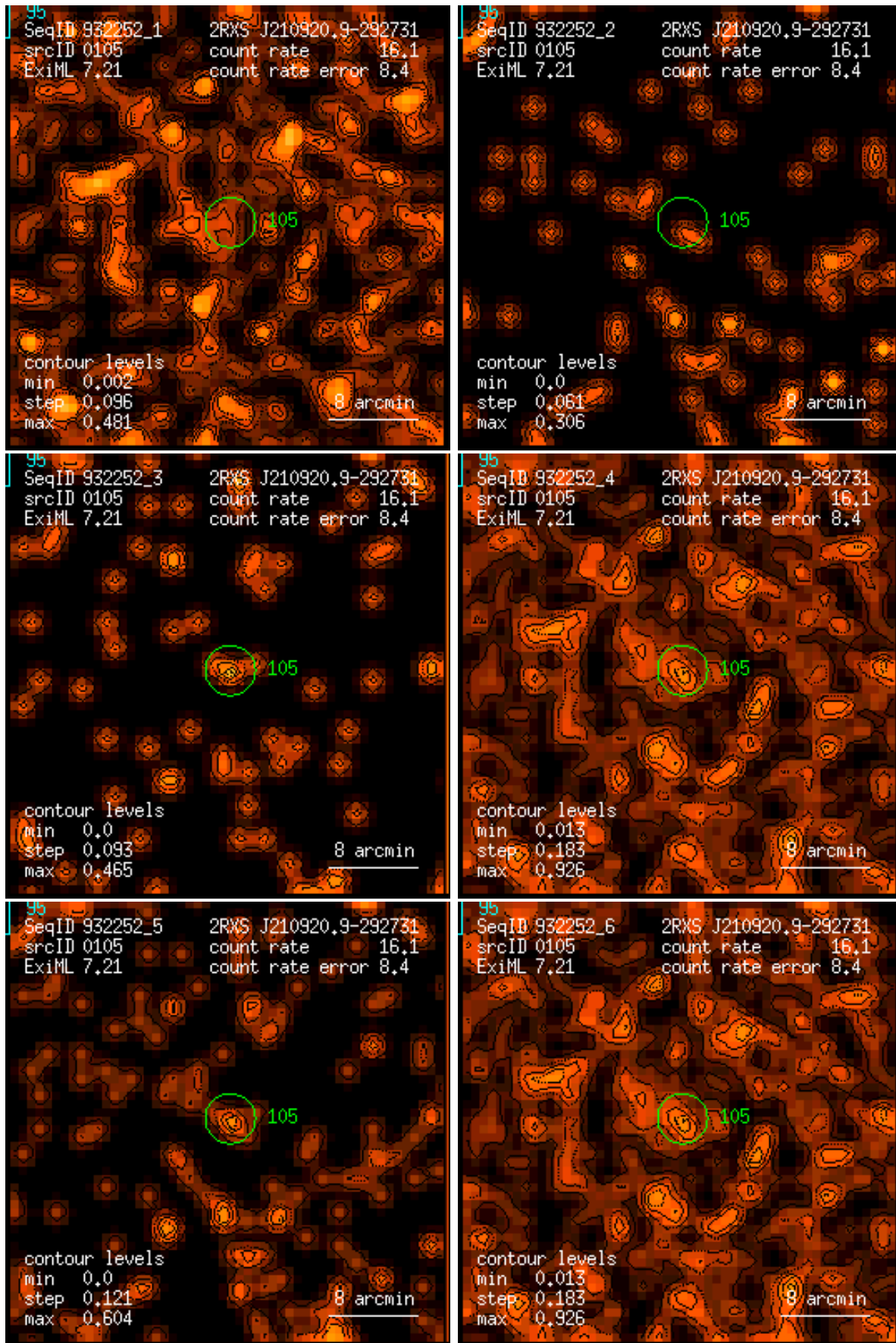
Figure 105: RASS 932252: detection 0105: band rate images, Gaussian filter: (1) PSPC channels 11 – 41, (2) 52 – 90, (3) 91 – 201, (4) 11 – 235, (5) 52 – 201, (6) 11 – 201. Broad band rates in counts/ks. Band rate contour levels in counts/ks/arcmin 2 .
