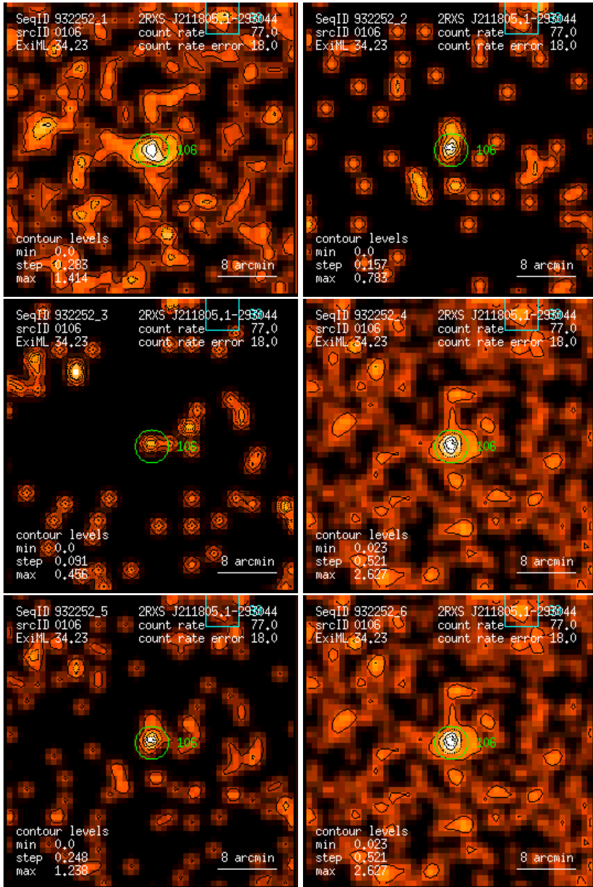
Figure 106: RASS 932252: detection 0106: band rate images, Gaussian filter: (1) PSPC channels 11 – 41, (2) 52 – 90, (3) 91 – 201, (4) 11 – 235, (5) 52 – 201, (6) 11 – 201. Broad band rates in counts/ks. Band rate contour levels in counts/ks/arcmin 2 .
