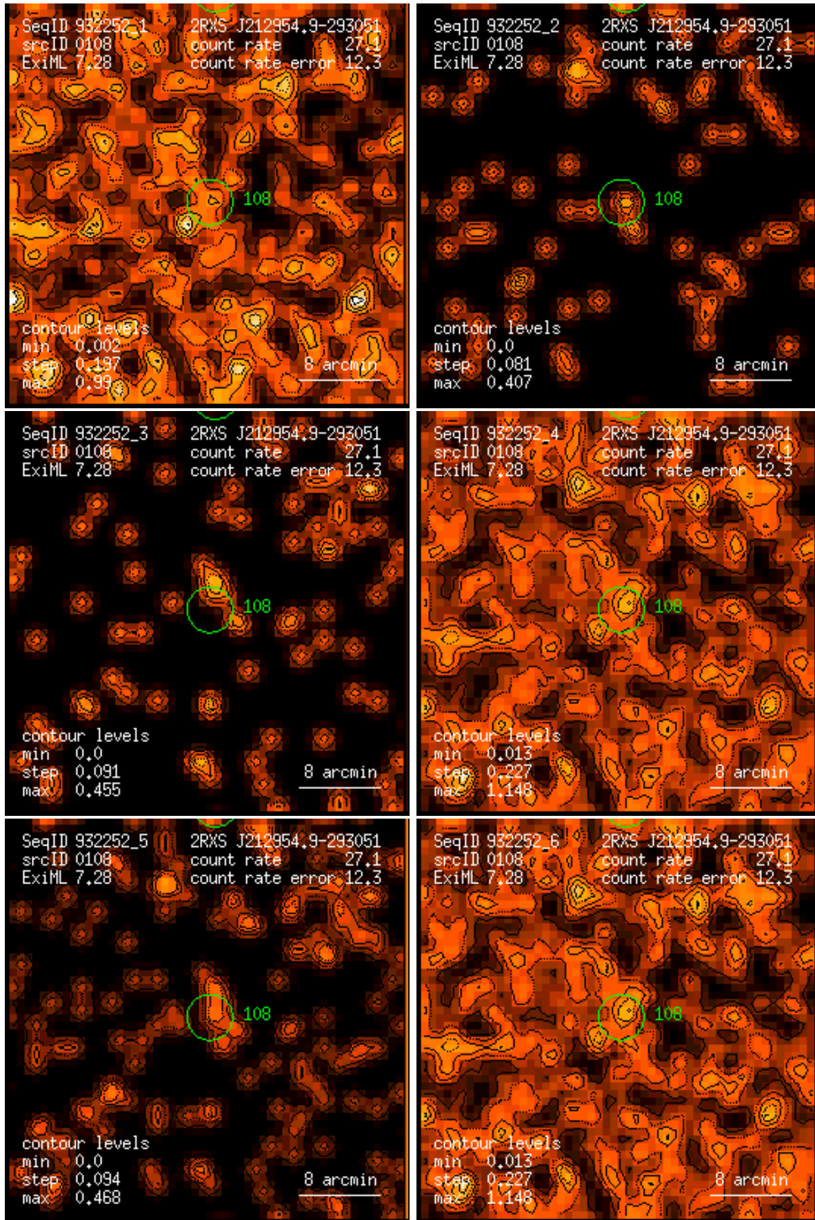
Figure 108: RASS 932252: detection 0108: band rate images, Gaussian filter: (1) PSPC channels 11 – 41, (2) 52 – 90, (3) 91 – 201, (4) 11 – 235, (5) 52 – 201, (6) 11 – 201. Broad band rates in counts/ks. Band rate contour levels in counts/ks/arcmin 2 .
